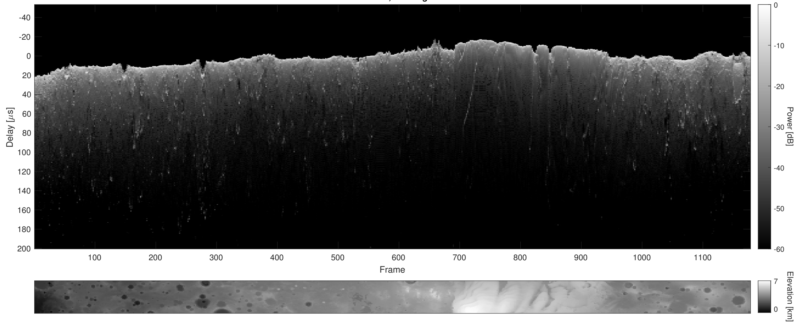
Orbit 10917, Cluttergram
