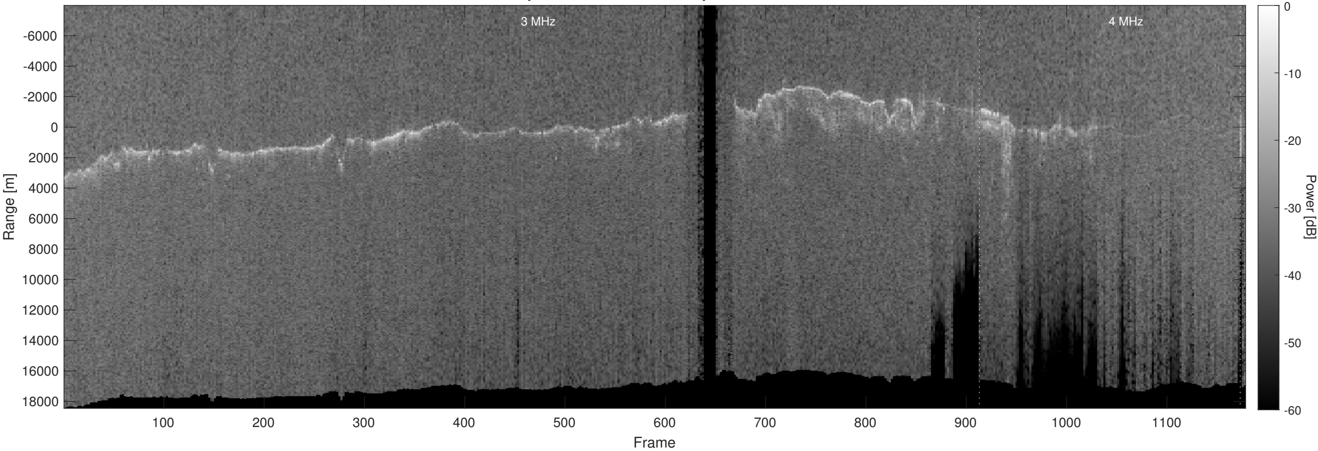
Orbit 10917, Optimized, No Window, Depth-Corrected, Channel 2
