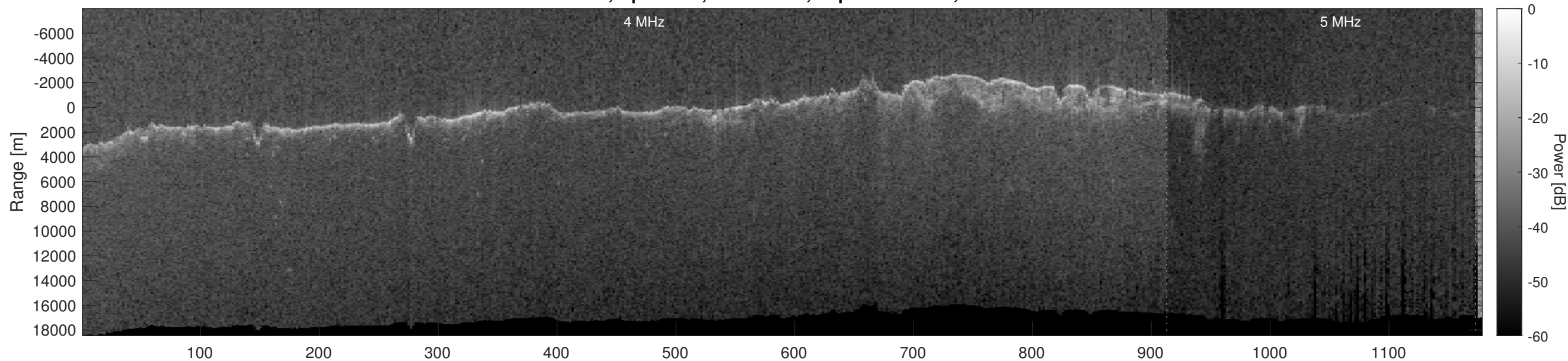
Orbit 10917, Optimized, No Window, Depth-Corrected, Channel 2
