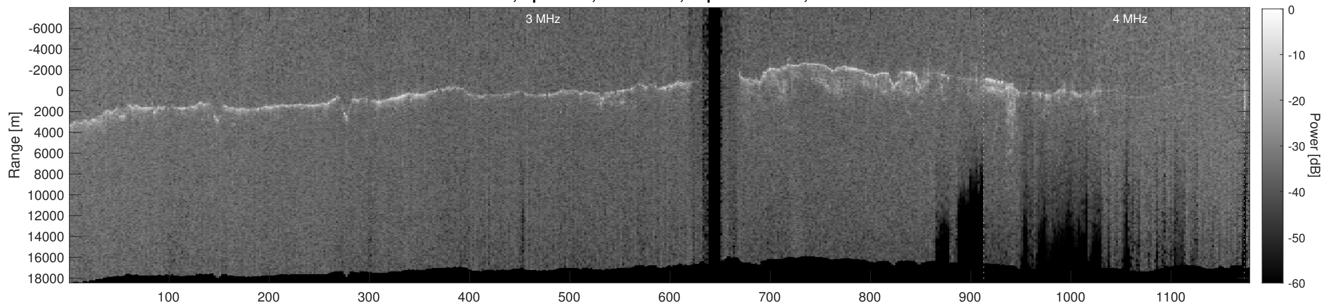
Orbit 10917, Depth-Corrected Cluttergram
