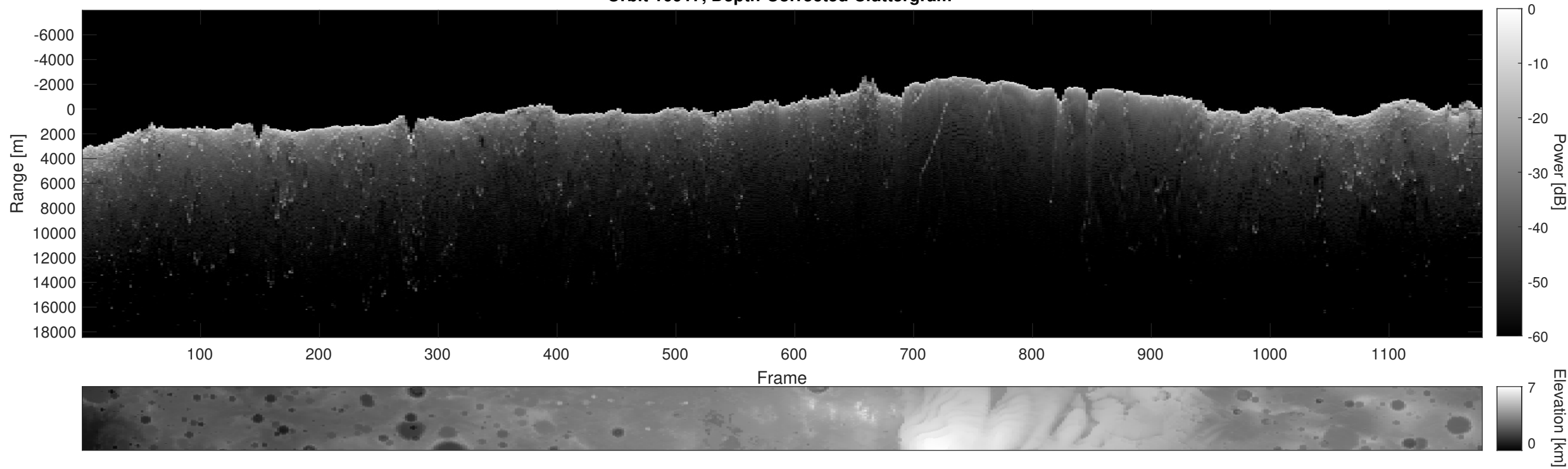
Orbit 10917, Depth-Corrected Cluttergram
