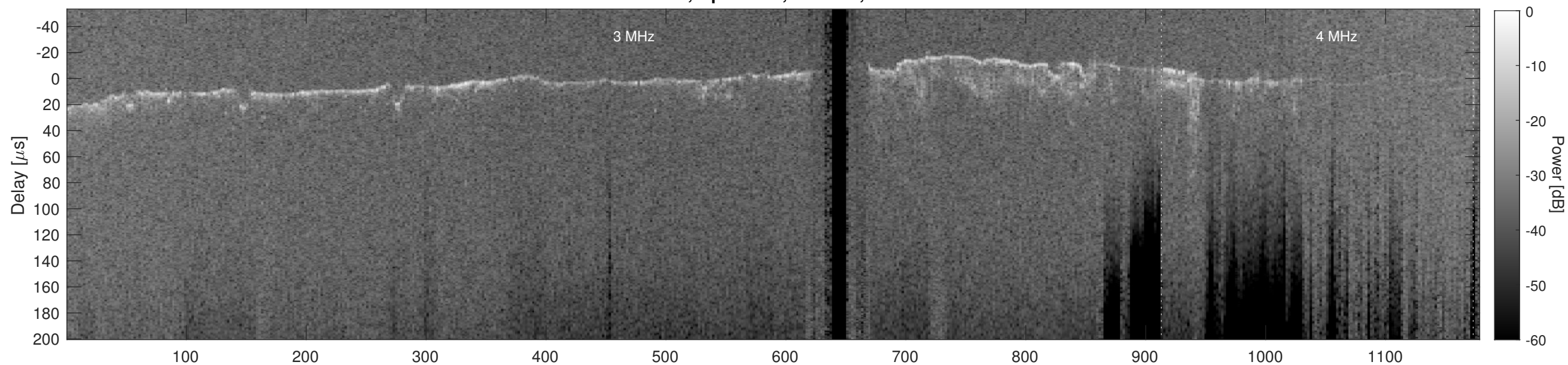
Orbit 10917, Cluttergram
