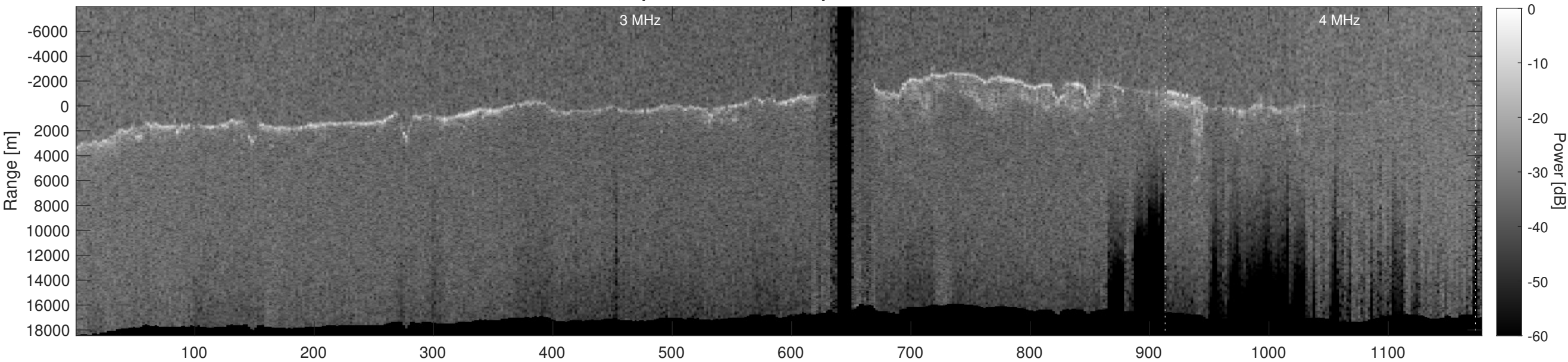
Orbit 10917, Depth-Corrected Cluttergram
