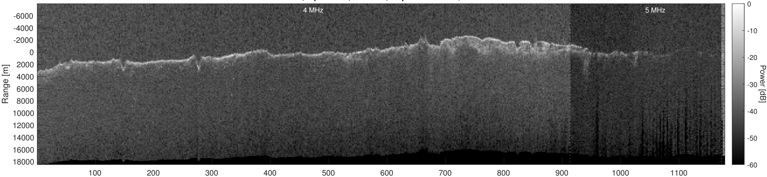
Orbit 10917, Optimized, Window, Depth-Corrected, Channel 2
