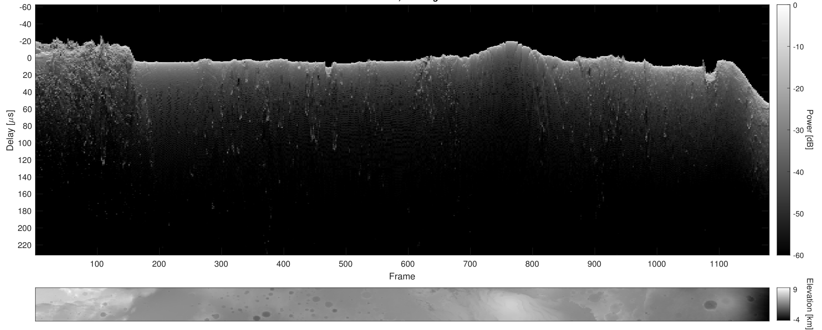
Orbit 10918, Cluttergram
