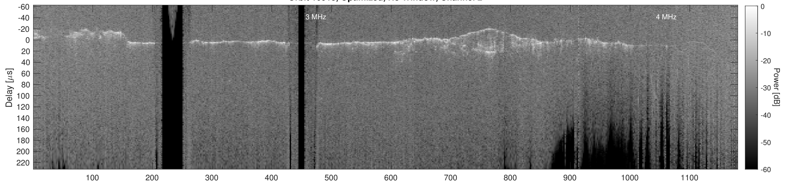
Orbit 10918, Cluttergram
