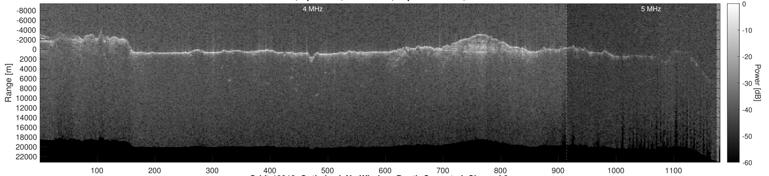
Orbit 10918, Optimized, No Window, Depth-Corrected, Channel 2
