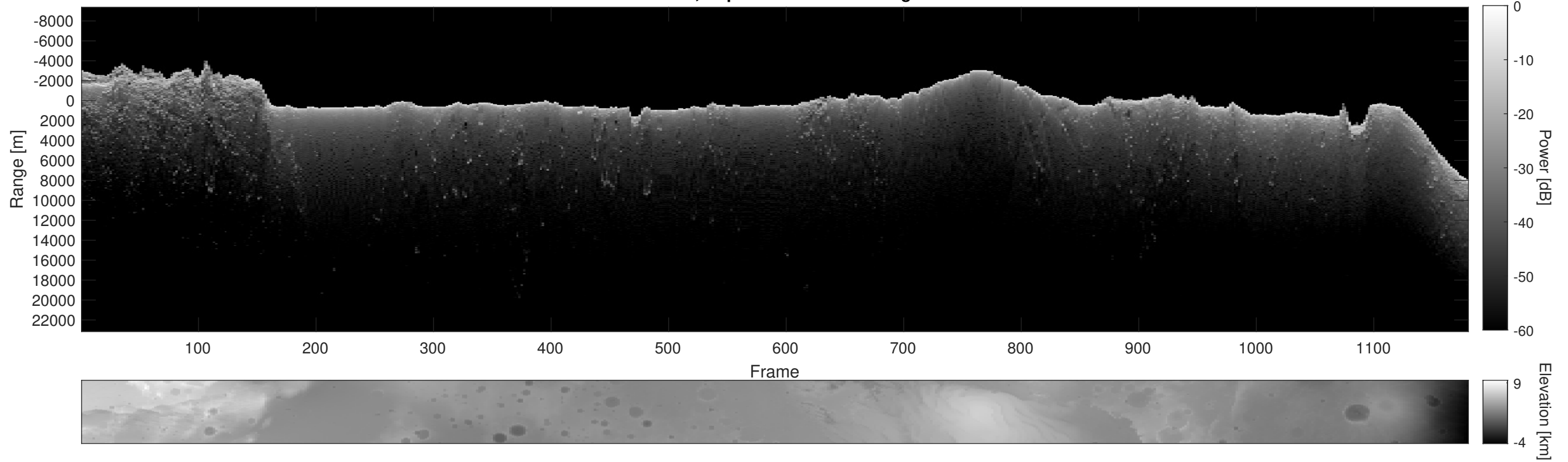
Orbit 10918, Depth-Corrected Cluttergram
