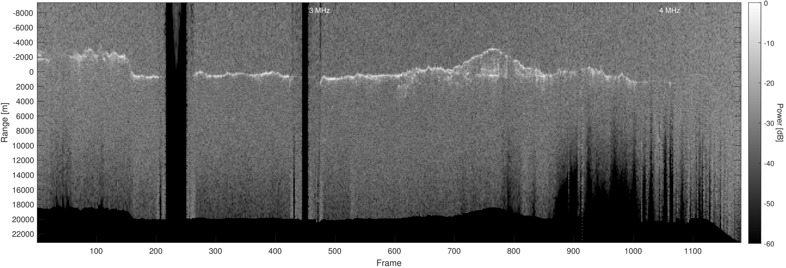
Orbit 10918, Optimized, Window, Depth-Corrected, Channel 2
