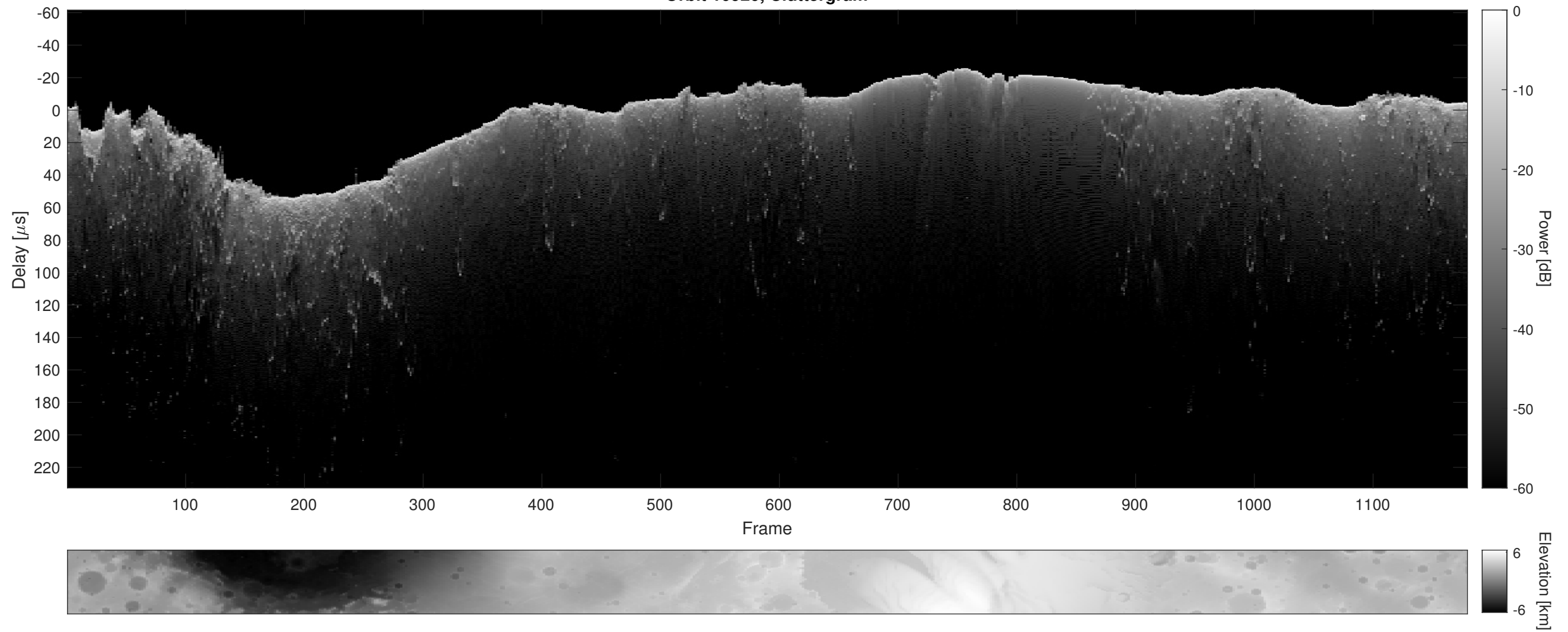
Orbit 10920, Cluttergram
