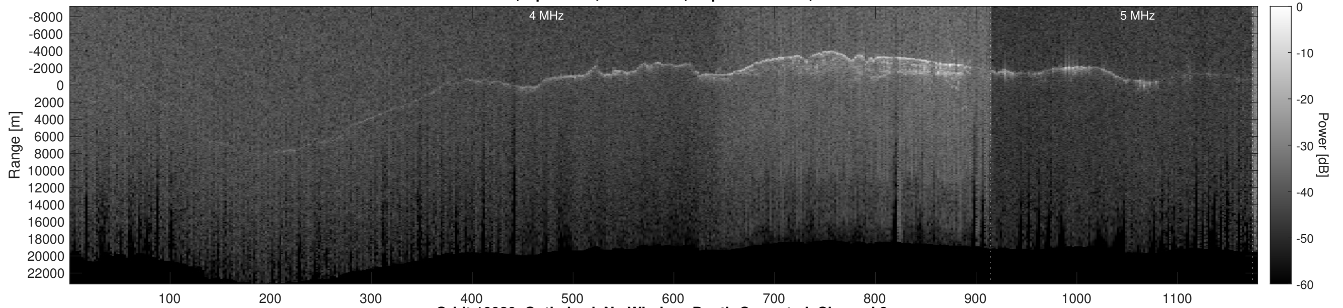
Orbit 10920, Optimized, No Window, Depth-Corrected, Channel 2
