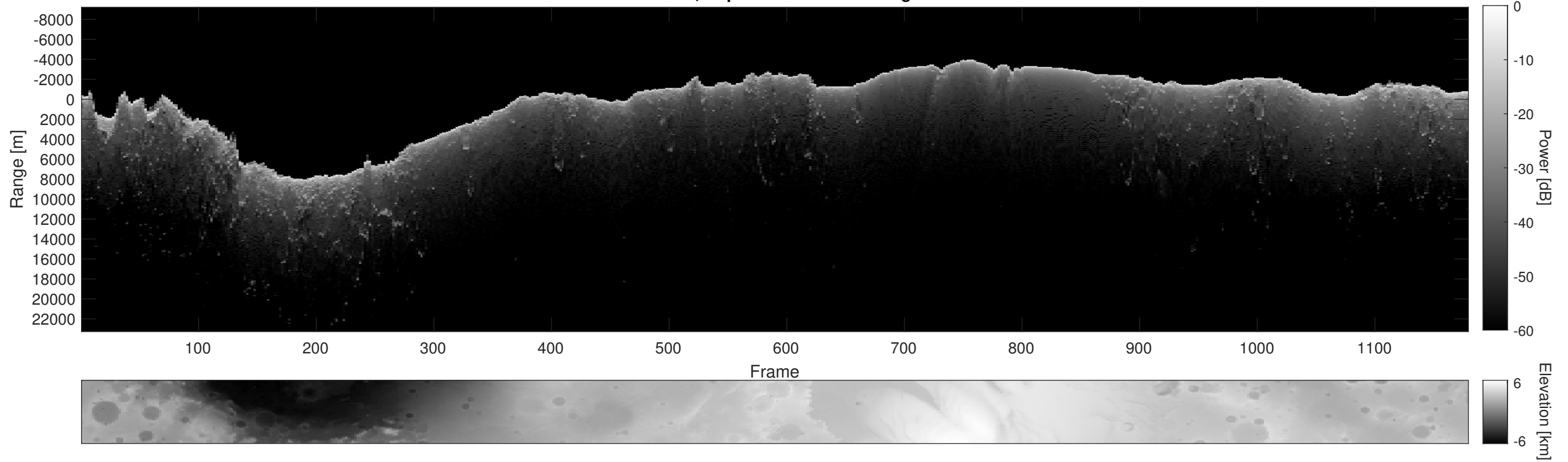
Orbit 10920, Depth-Corrected Cluttergram
