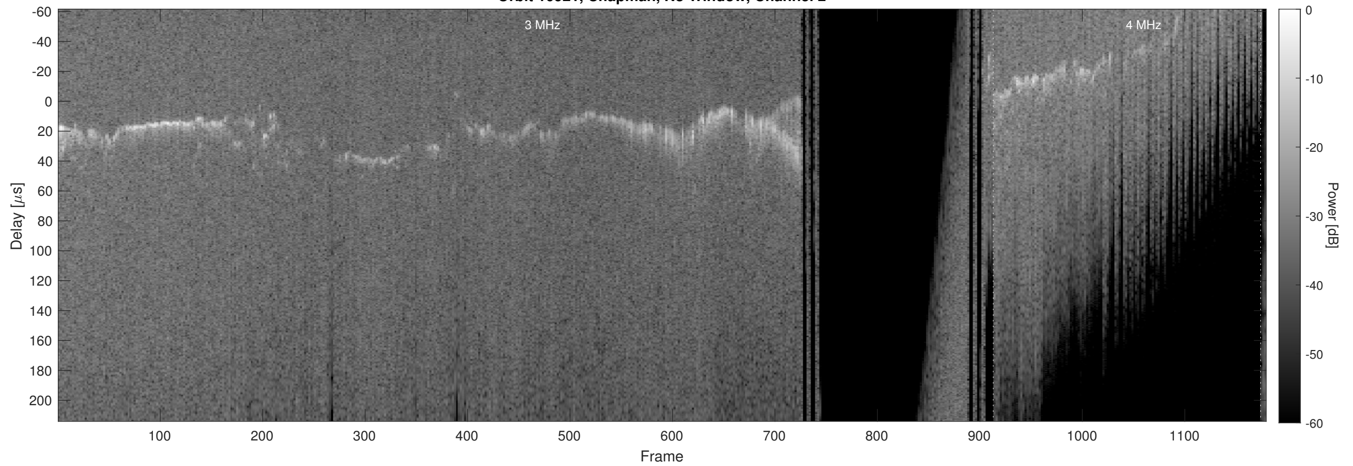
Orbit 10921, Chapman, No Window, Channel 2
