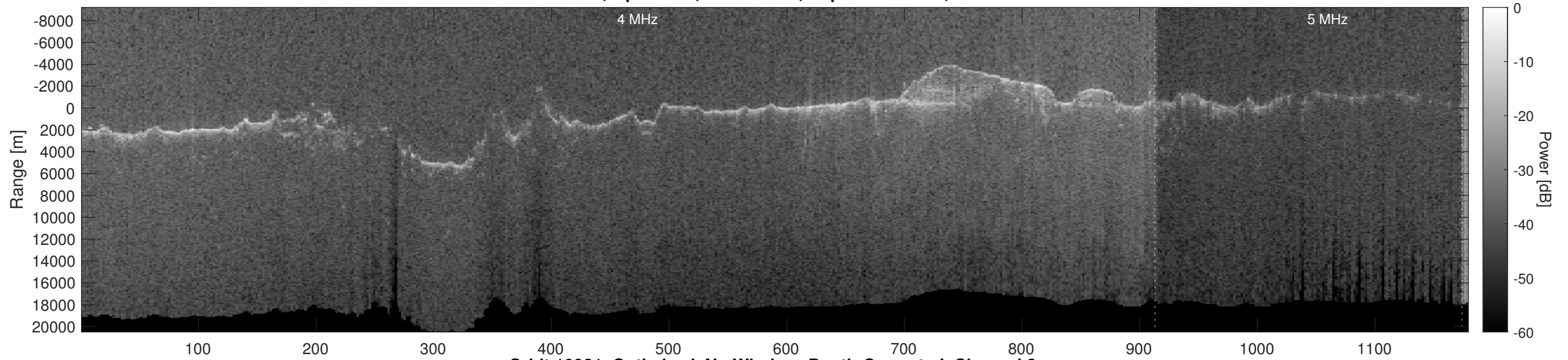
Orbit 10921, Optimized, No Window, Depth-Corrected, Channel 2
