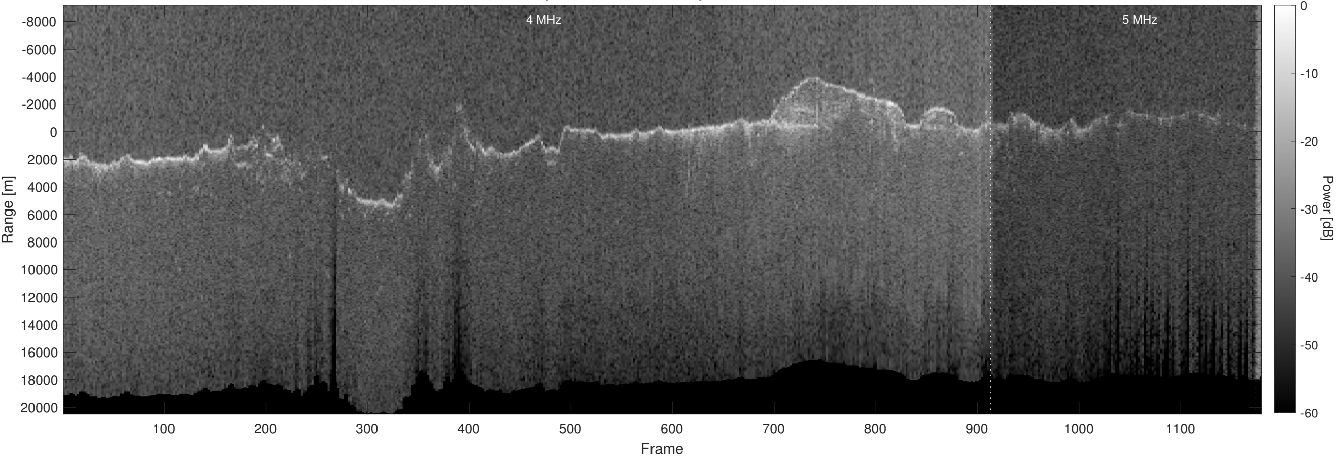
Orbit 10921, Optimized, Window, Depth-Corrected, Channel 2
