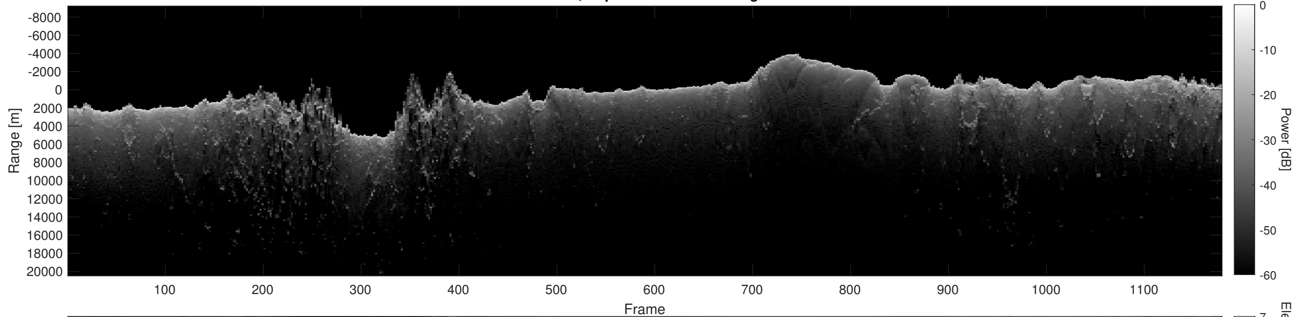
Orbit 10921, Depth-Corrected Cluttergram
