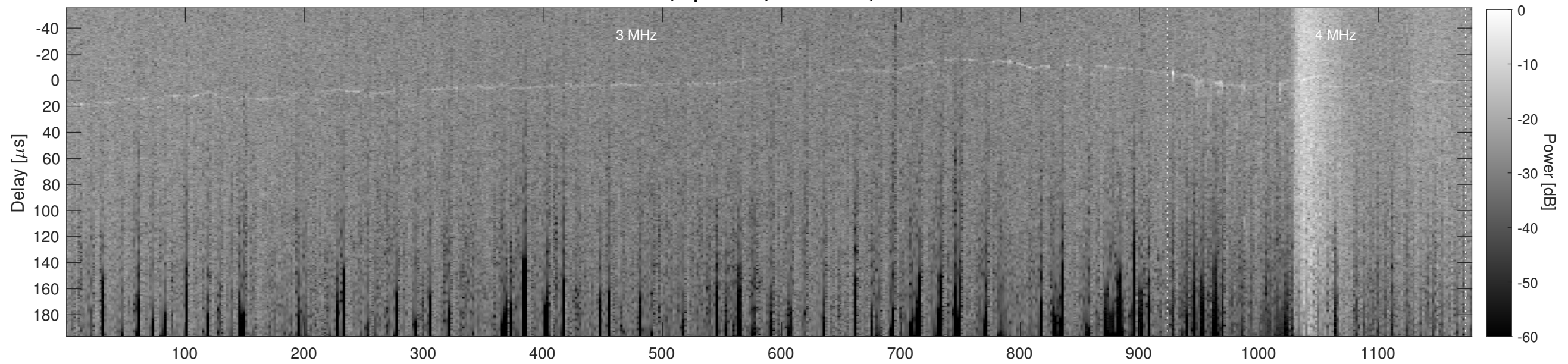
Orbit 10924, Cluttergram
