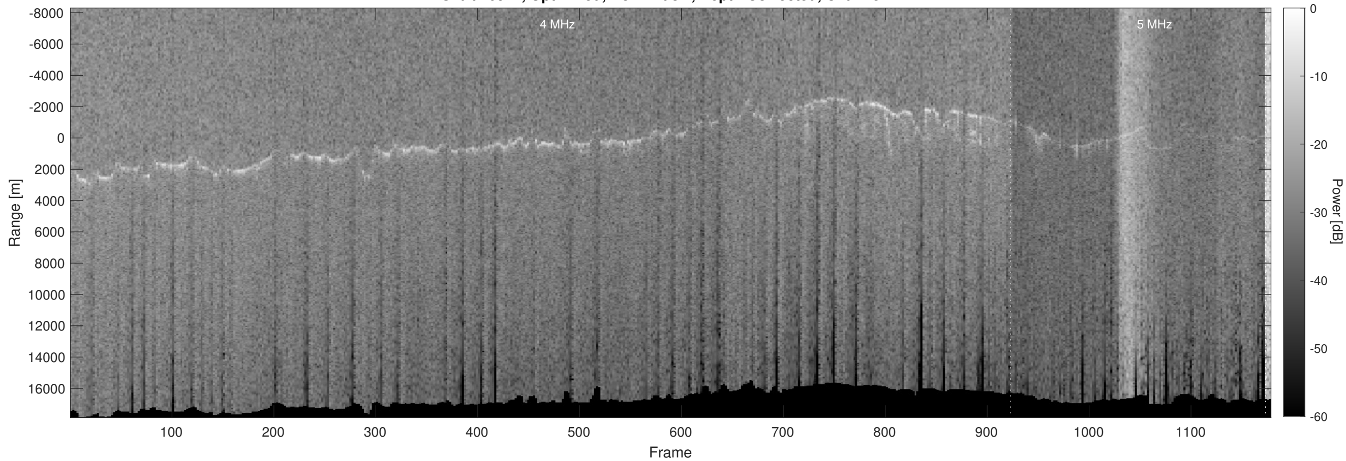
Orbit 10924, Optimized, No Window, Depth-Corrected, Channel 2
