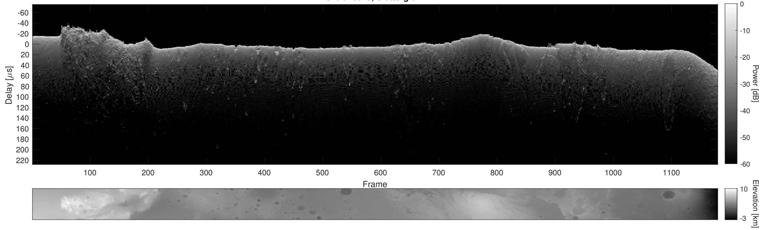
Orbit 10925, Cluttergram
