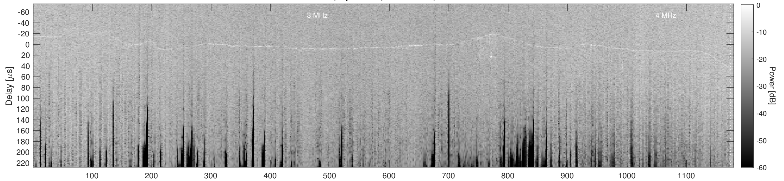
Orbit 10925, Cluttergram
