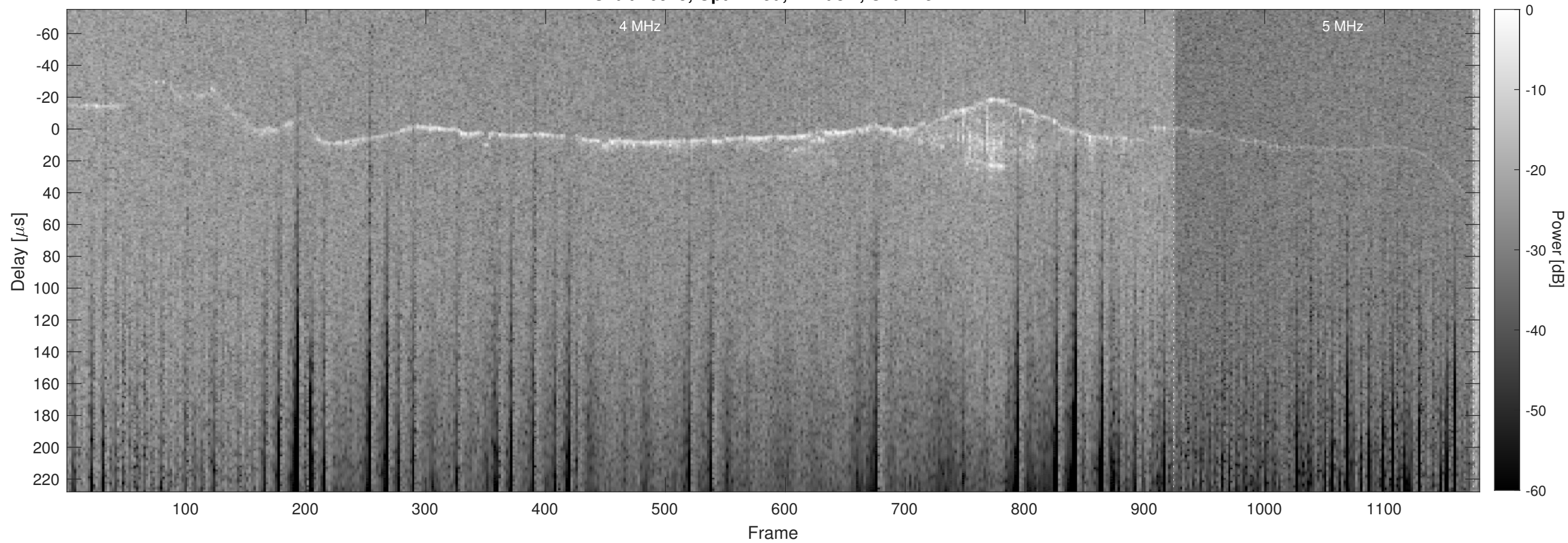
Orbit 10925, Optimized, Window, Channel 2
