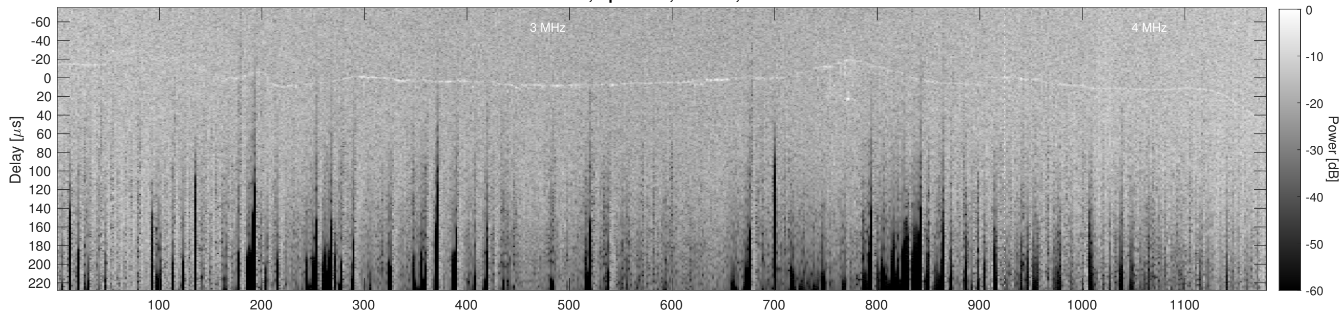
Orbit 10925, Cluttergram
