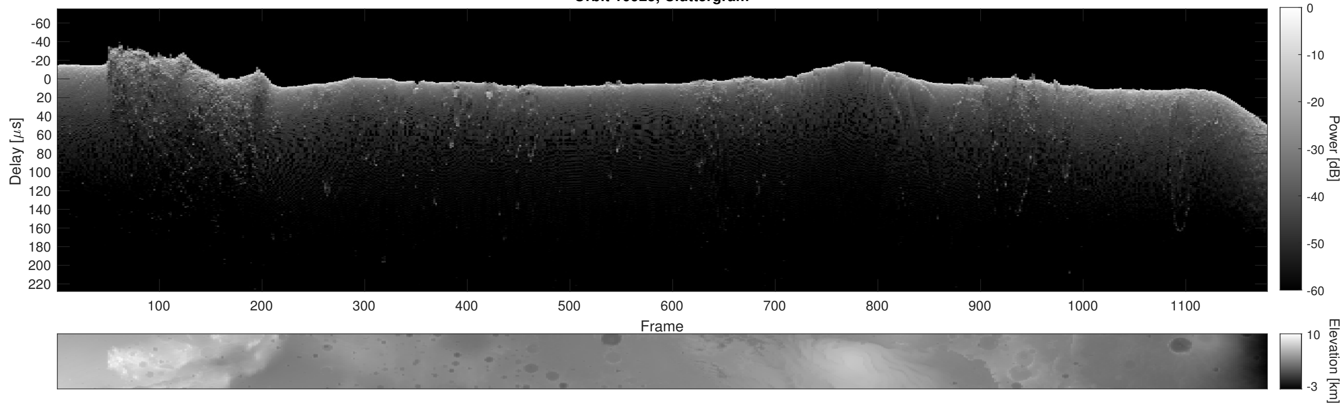
Orbit 10925, Cluttergram
