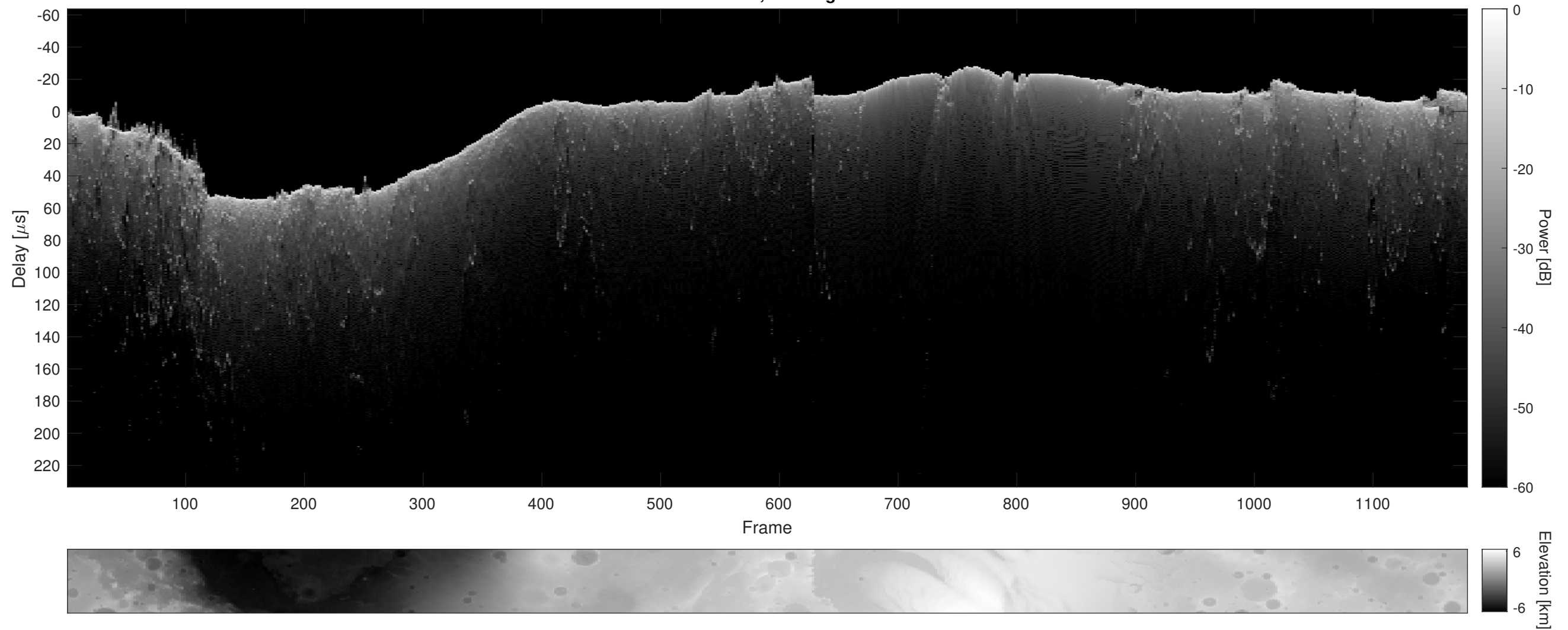
Orbit 10927, Cluttergram
