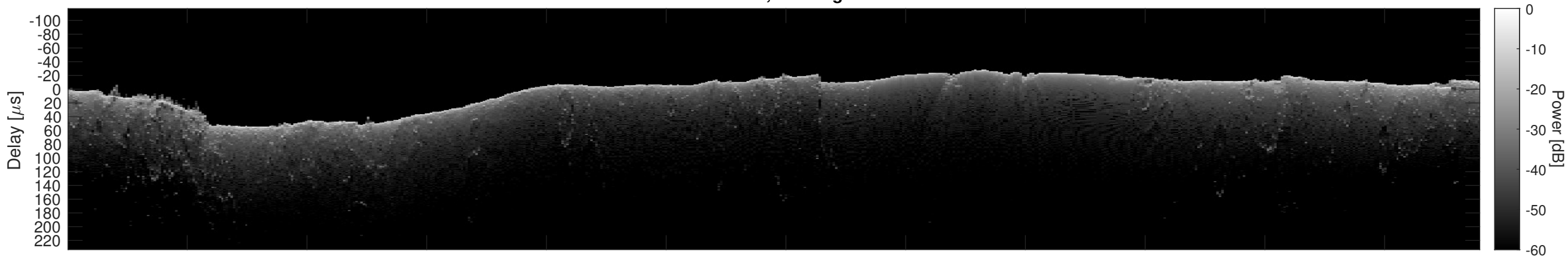
Orbit 10927, Cluttergram
