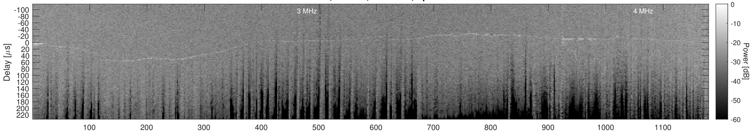
Orbit 10927, Cluttergram
