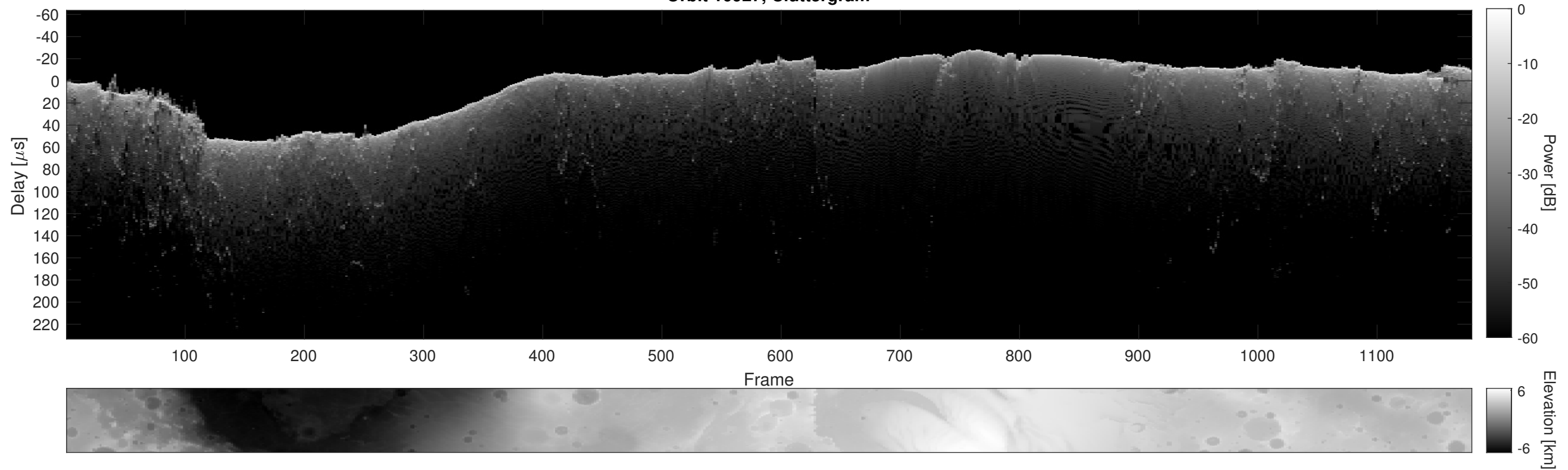
Orbit 10927, Cluttergram
