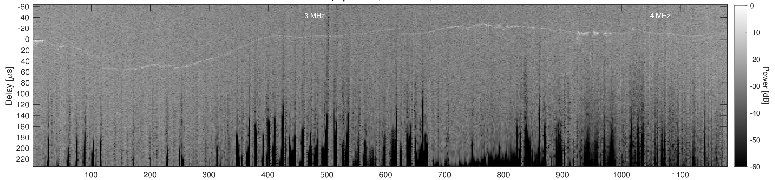
Orbit 10927, Cluttergram
