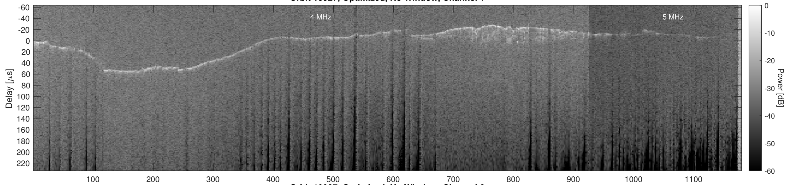
Orbit 10927, Optimized, No Window, Channel 2
