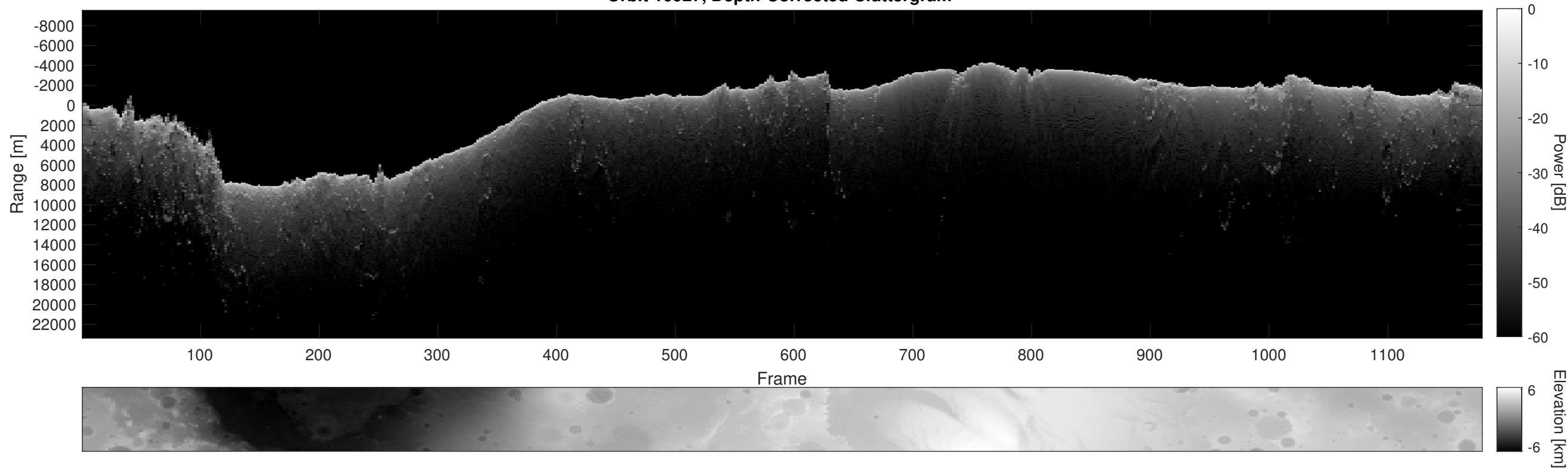
Orbit 10927, Depth-Corrected Cluttergram
