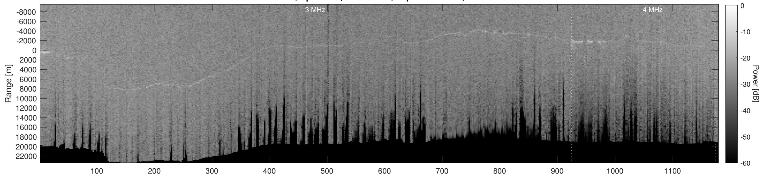
Orbit 10927, Depth-Corrected Cluttergram
