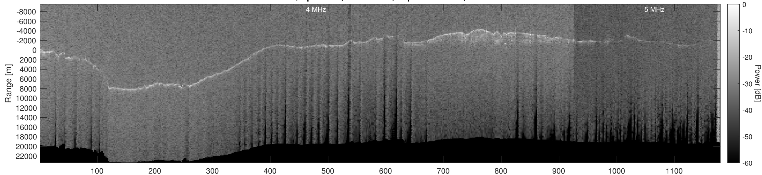
Orbit 10927, Optimized, No Window, Depth-Corrected, Channel 2
