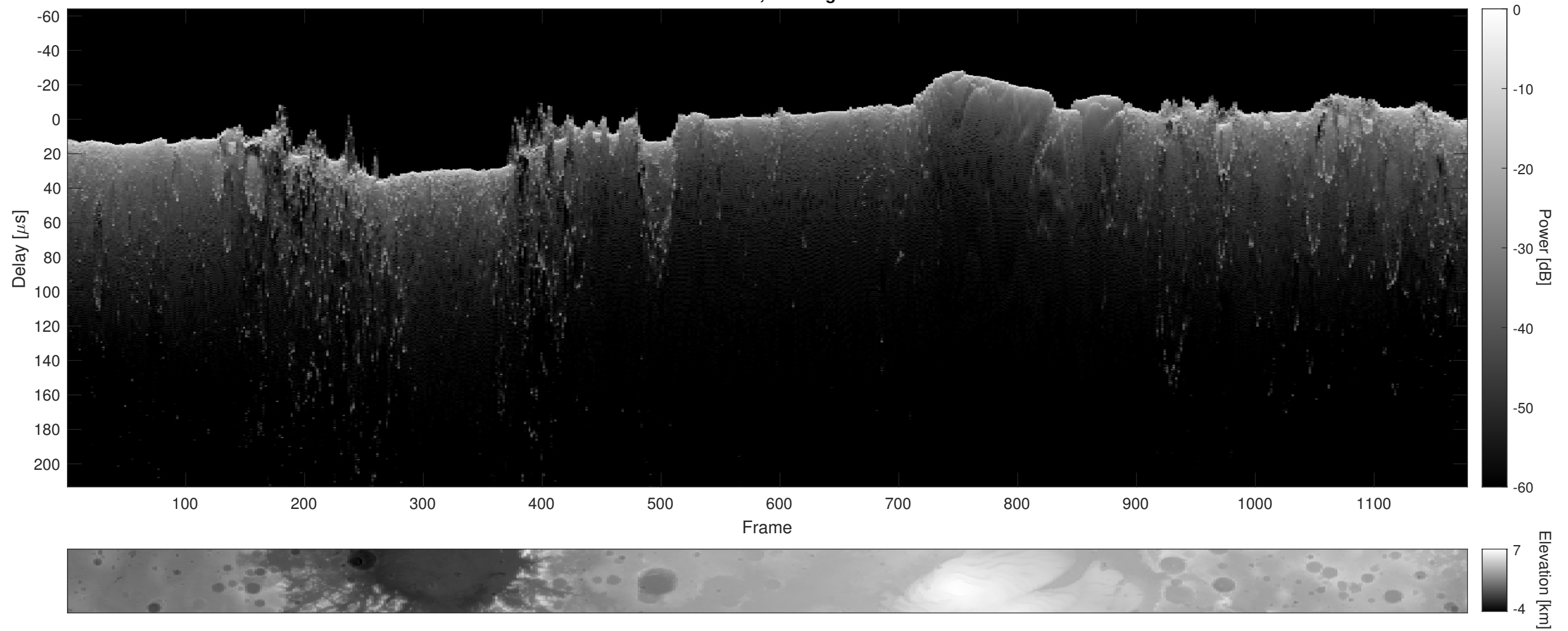
Orbit 10928, Cluttergram
