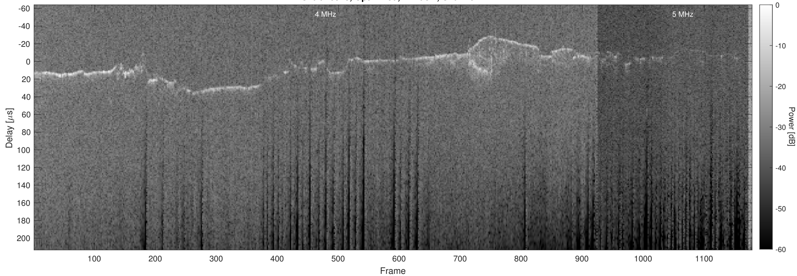
Orbit 10928, Optimized, Window, Channel 2
