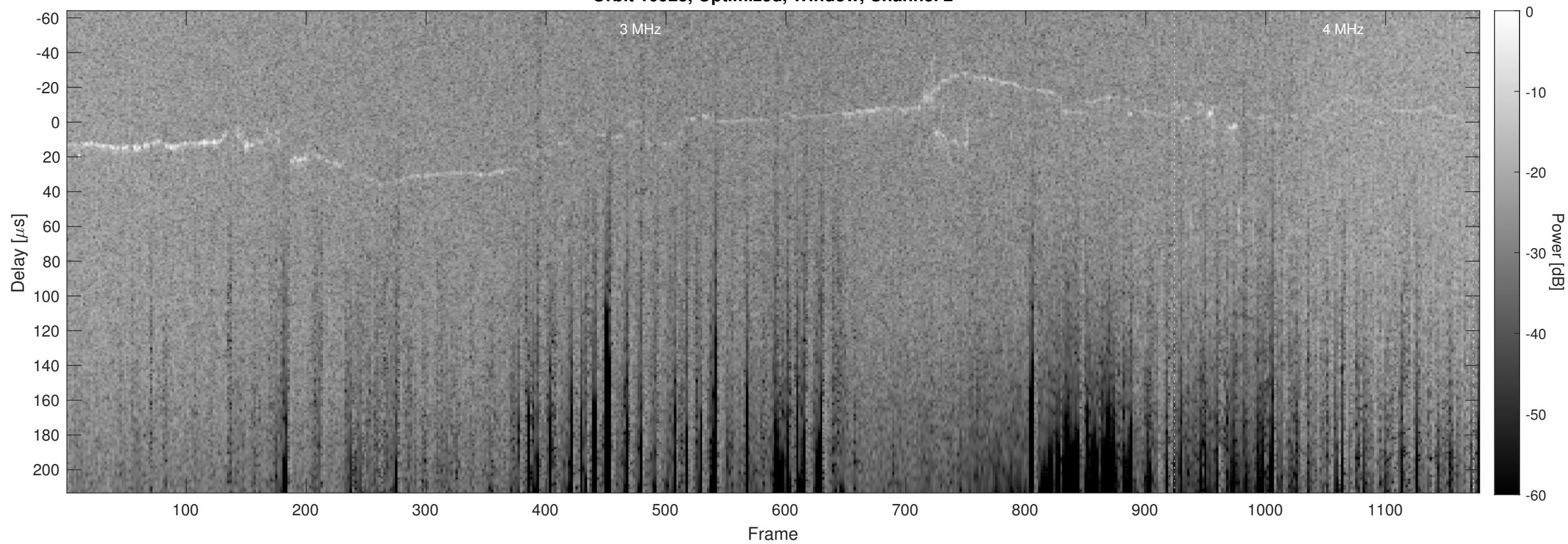
Orbit 10928, Optimized, Window, Channel 2
