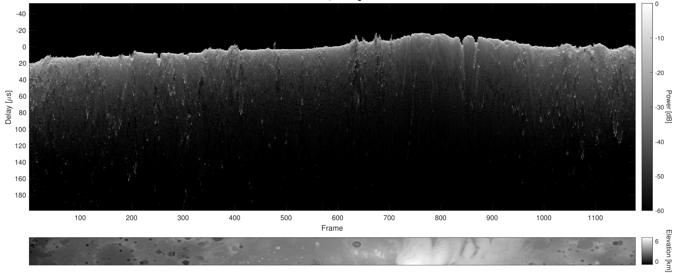
Orbit 10931, Cluttergram
