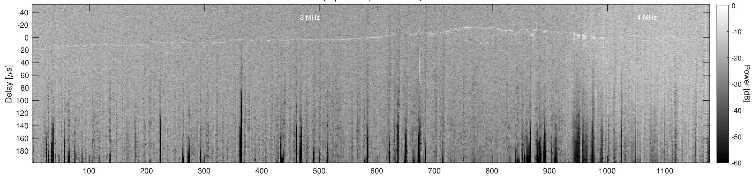
Orbit 10931, Cluttergram
