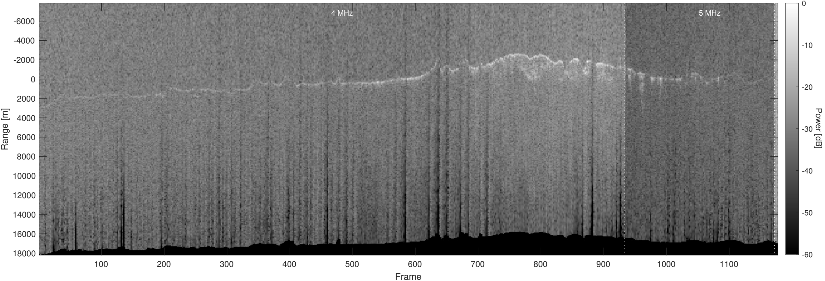
Orbit 10931, Optimized, No Window, Depth-Corrected, Channel 2
