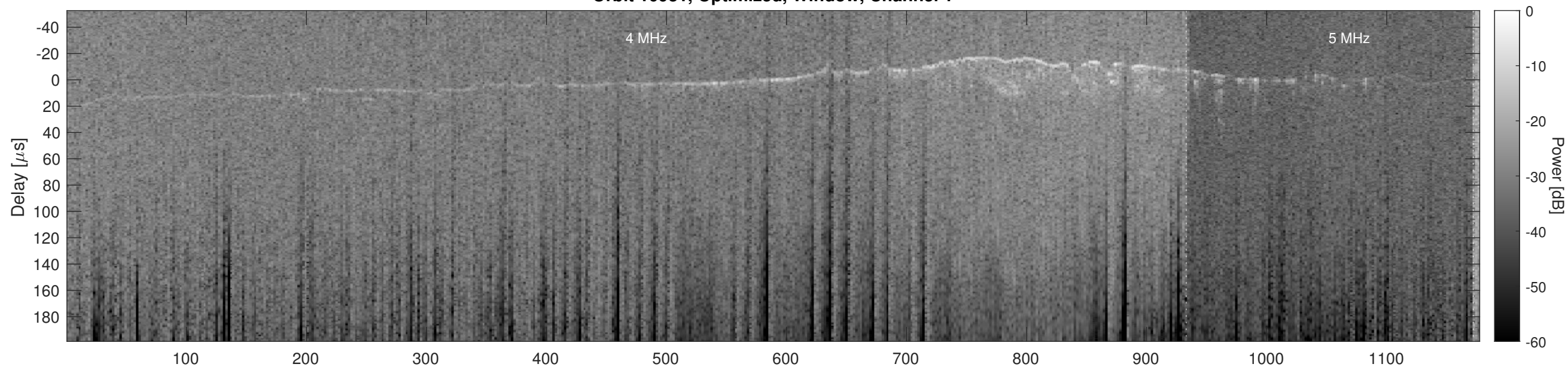
Orbit 10931, Optimized, Window, Channel 2
