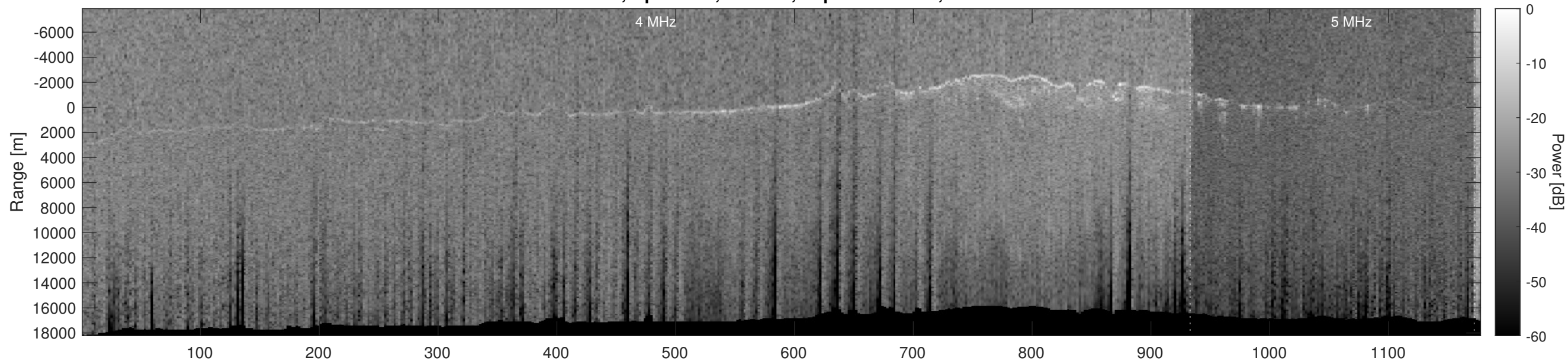
Orbit 10931, Optimized, Window, Depth-Corrected, Channel 2
