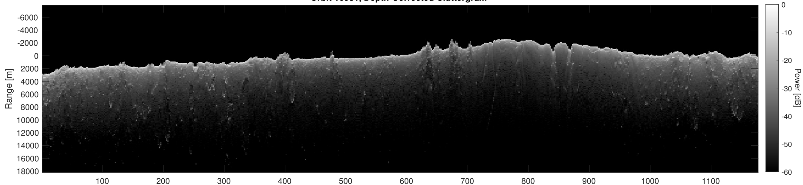
Orbit 10931, Depth-Corrected Cluttergram
