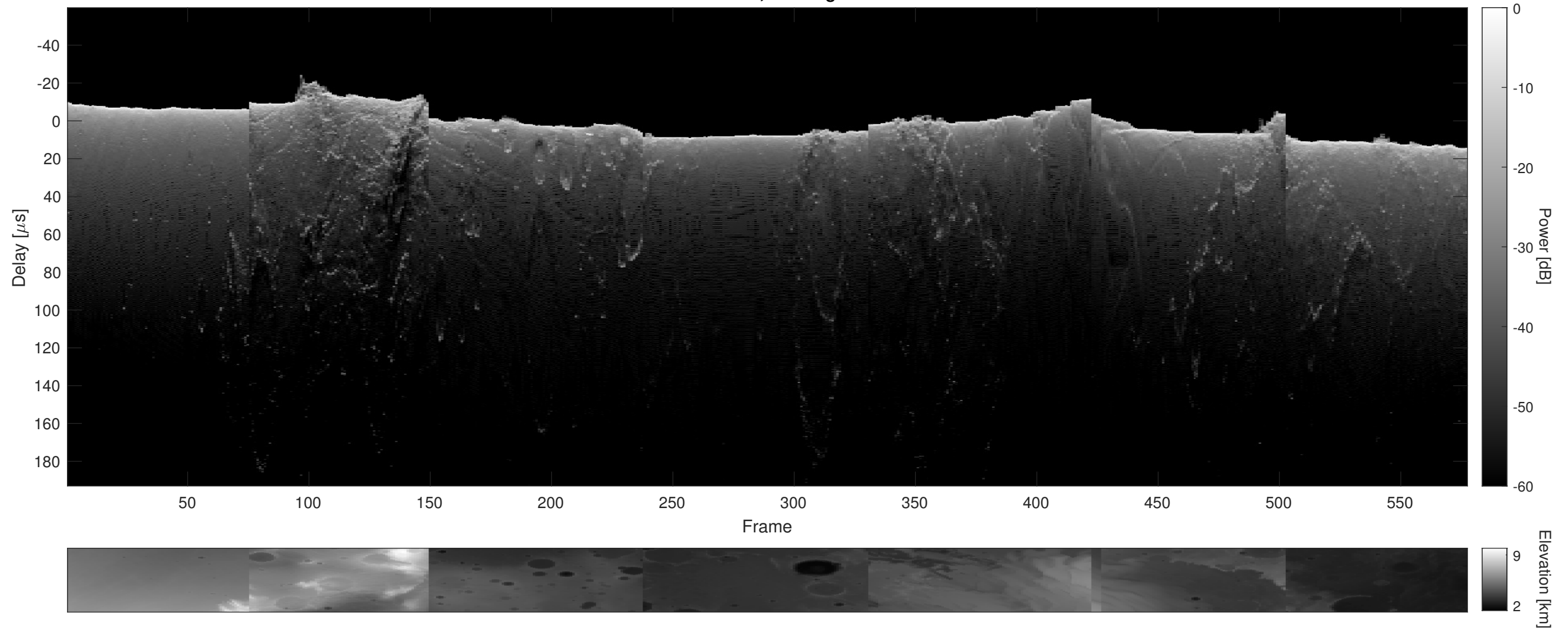
Orbit 10932, Cluttergram
