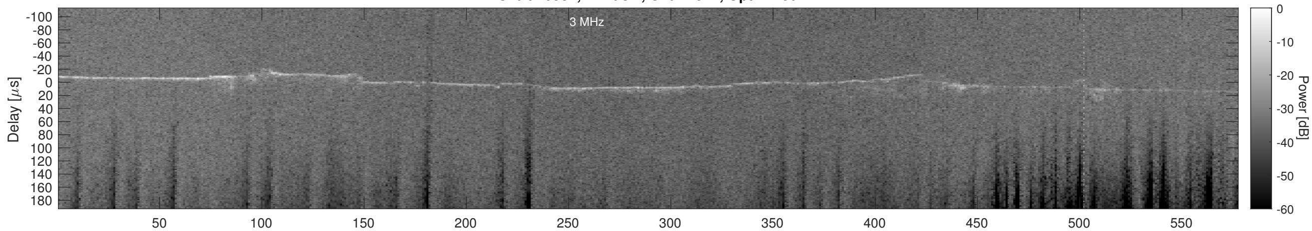
Orbit 10932, Cluttergram
