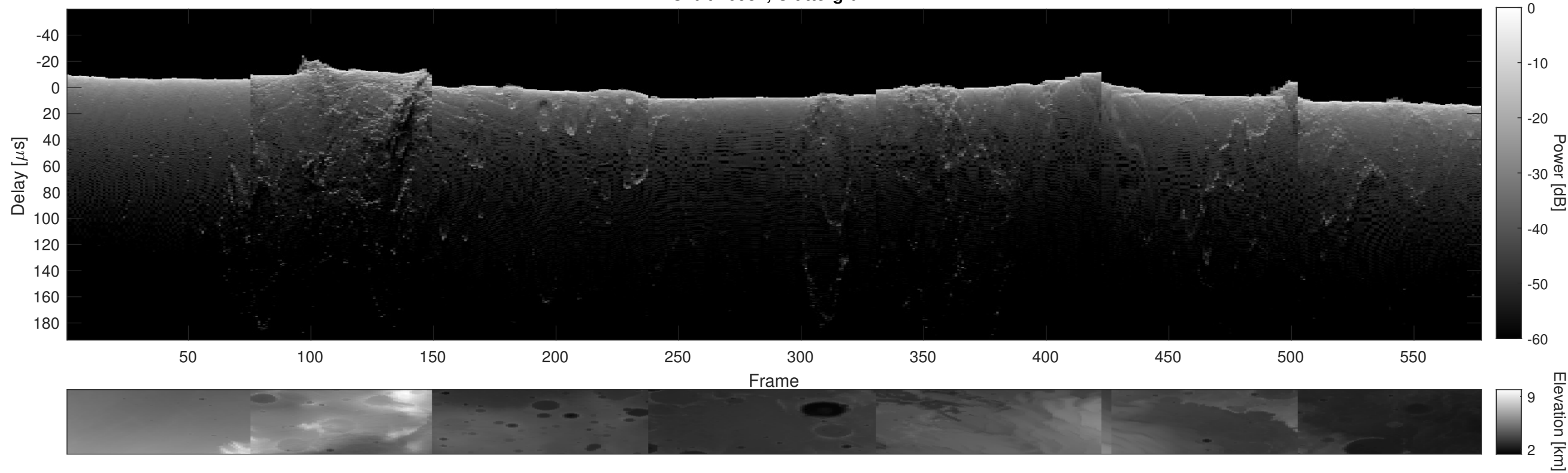
Orbit 10932, Cluttergram
