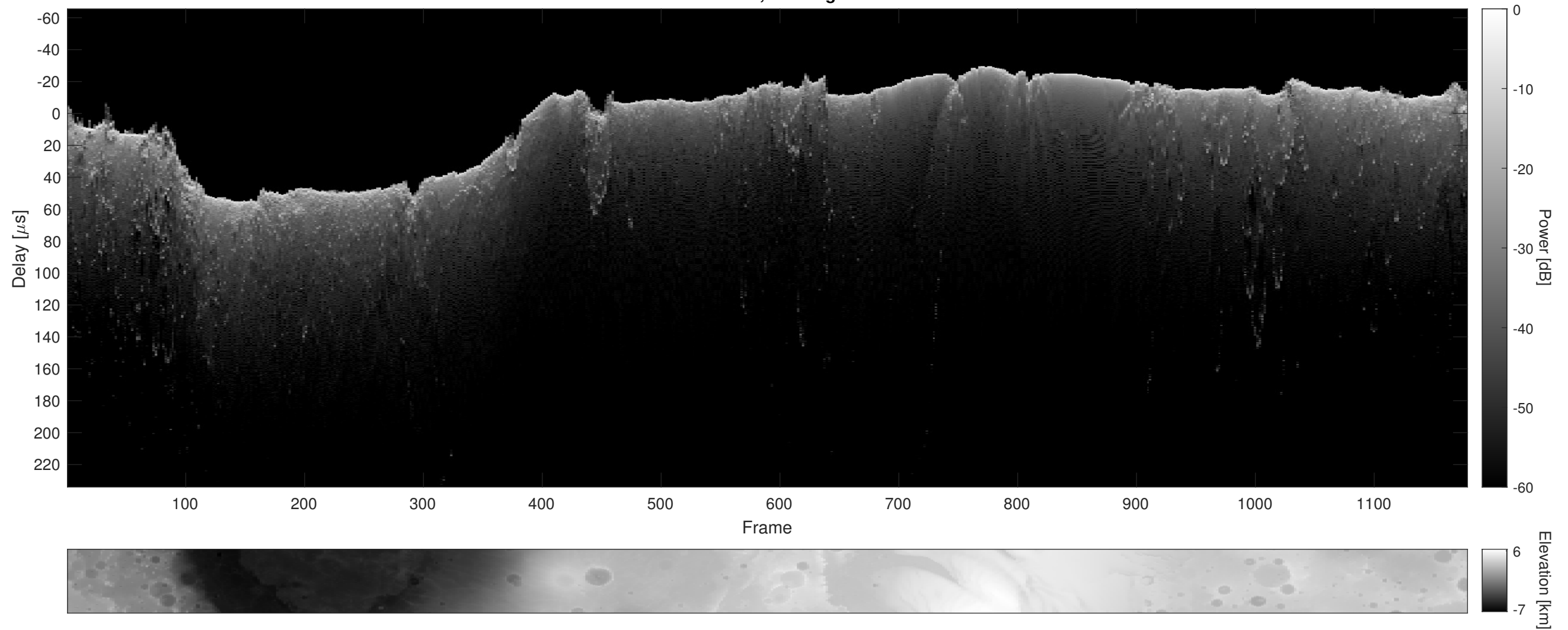
Orbit 10934, Cluttergram
