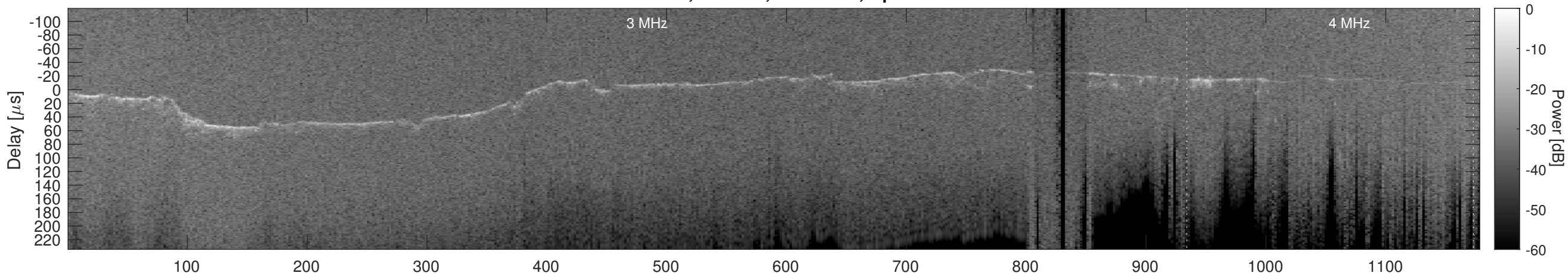
Orbit 10934, Cluttergram
