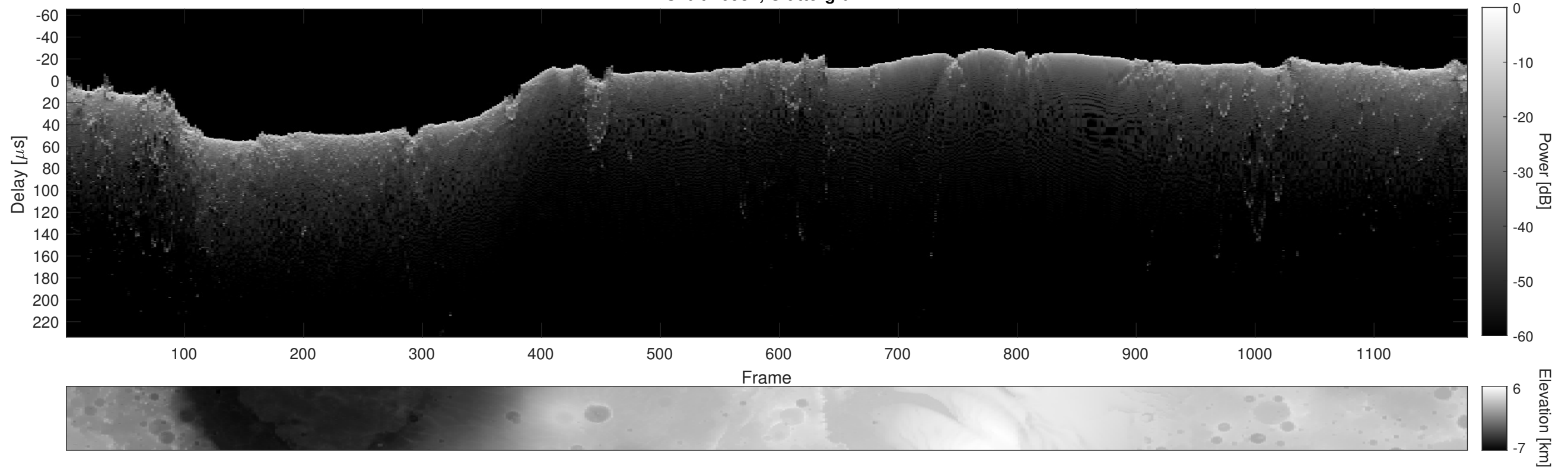
Orbit 10934, Cluttergram
