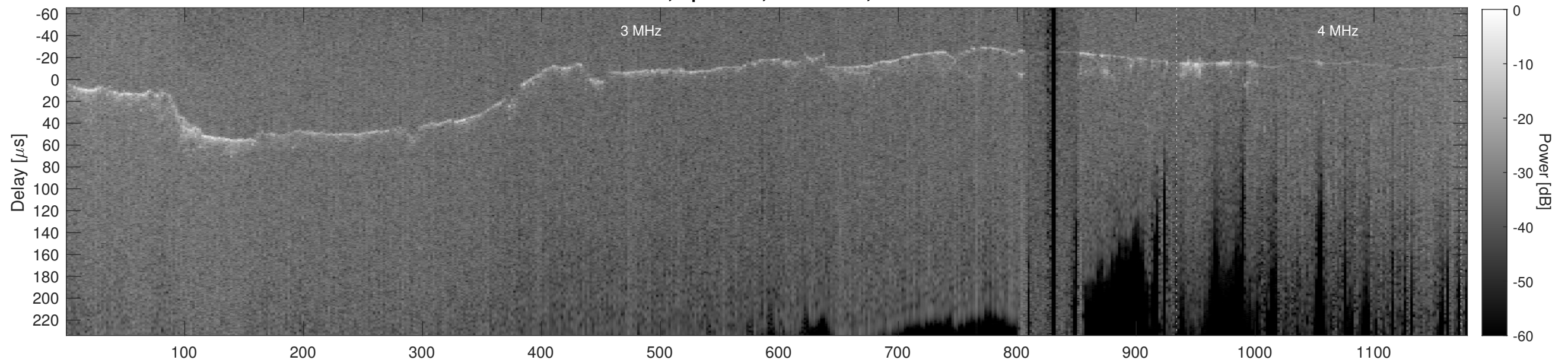
Orbit 10934, Cluttergram
