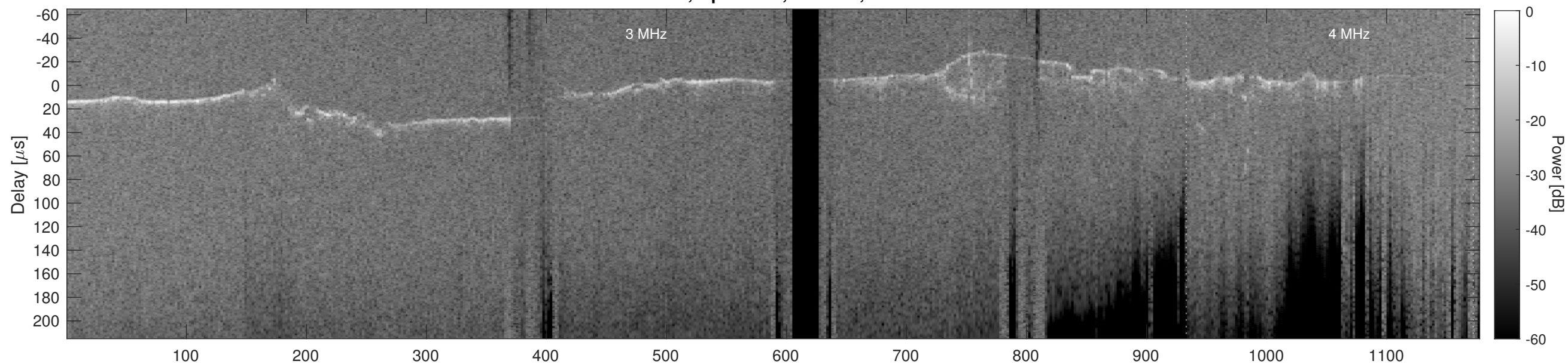
Orbit 10935, Cluttergram
