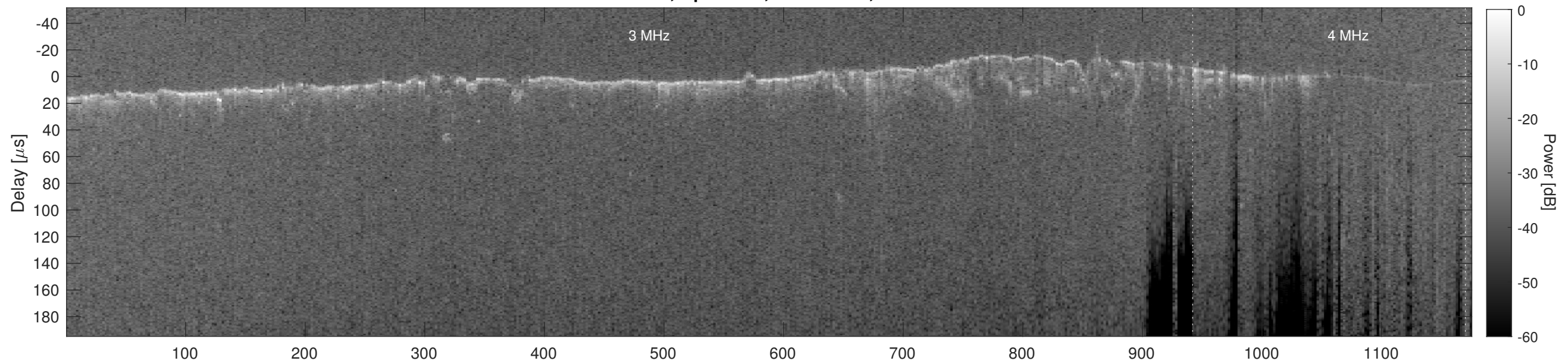
Orbit 10938, Cluttergram
