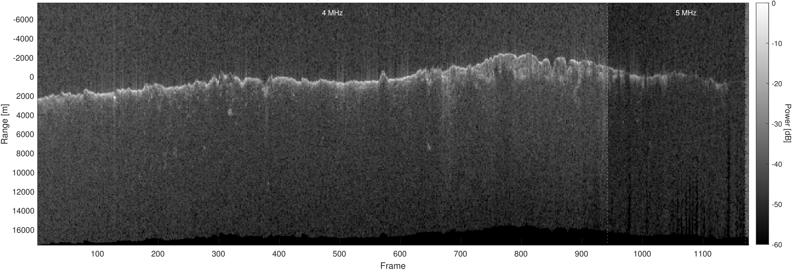
Orbit 10938, Optimized, No Window, Depth-Corrected, Channel 2
