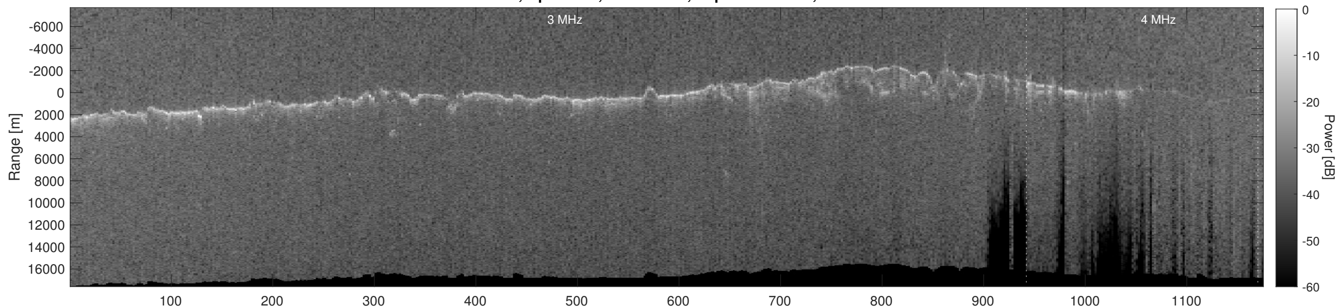
Orbit 10938, Depth-Corrected Cluttergram
