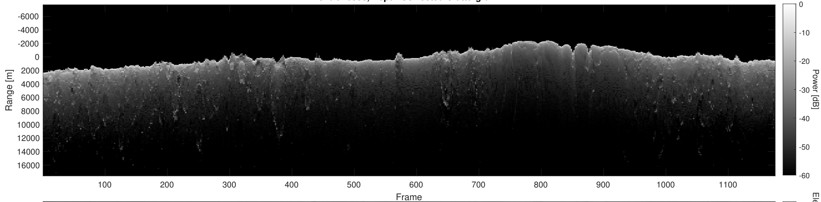
Orbit 10938, Depth-Corrected Cluttergram
