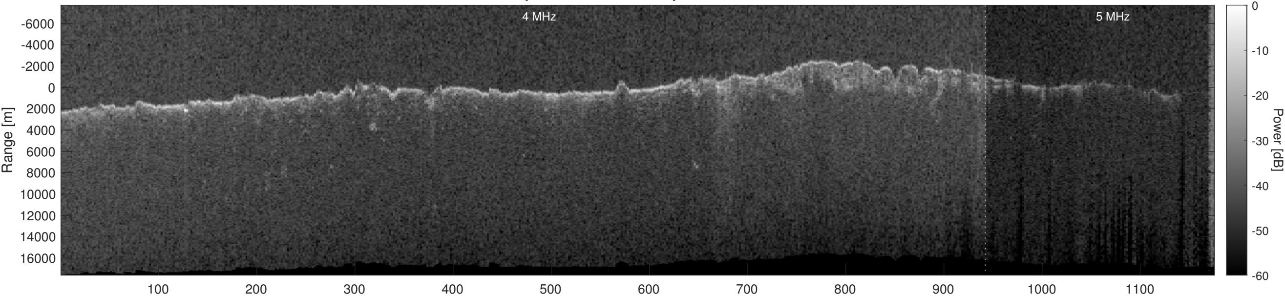
Orbit 10938, Optimized, Window, Depth-Corrected, Channel 2
