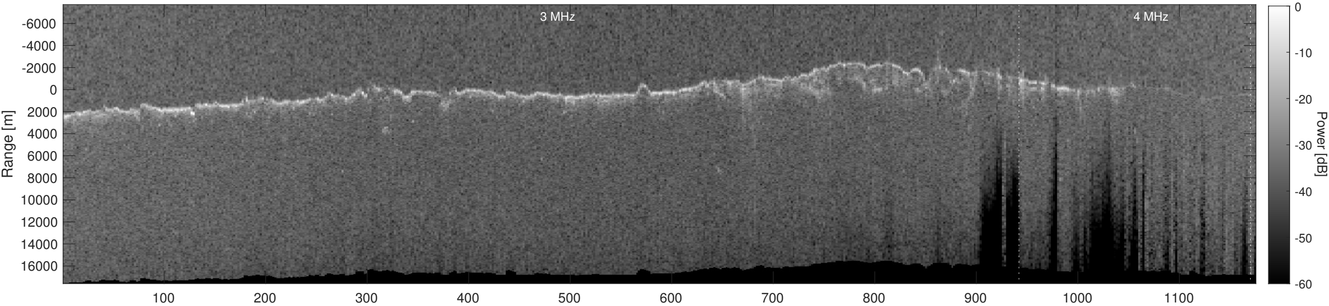
Orbit 10938, Depth-Corrected Cluttergram
