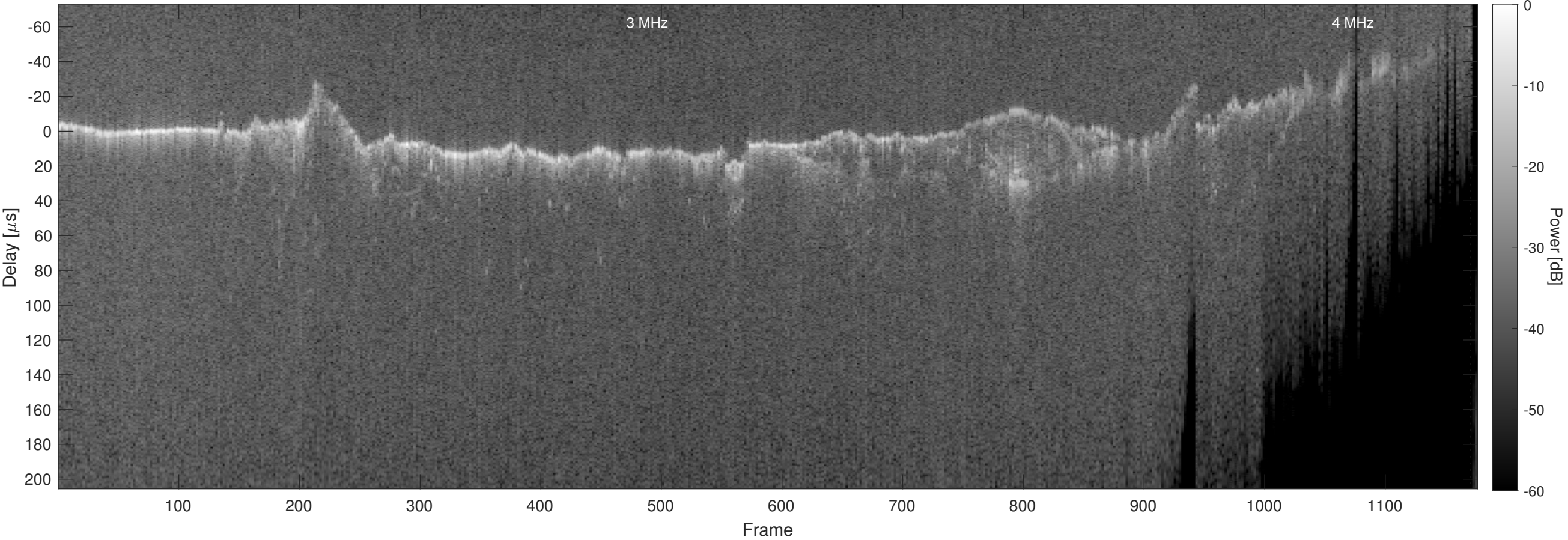
Orbit 10939, Chapman, No Window, Channel 2
