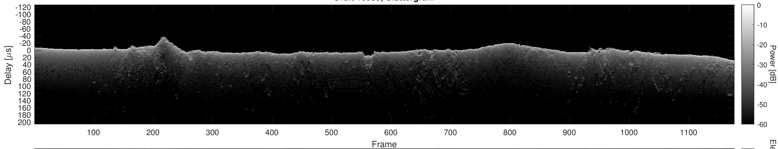
Orbit 10939, Cluttergram
