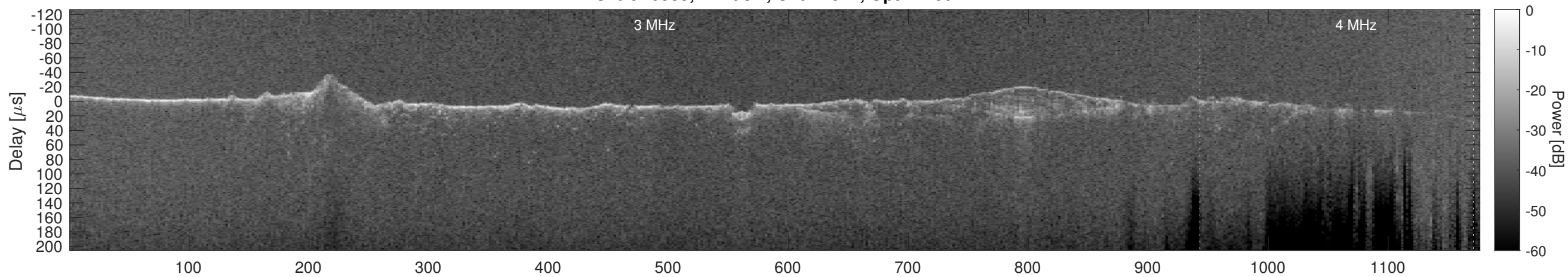
Orbit 10939, Cluttergram
