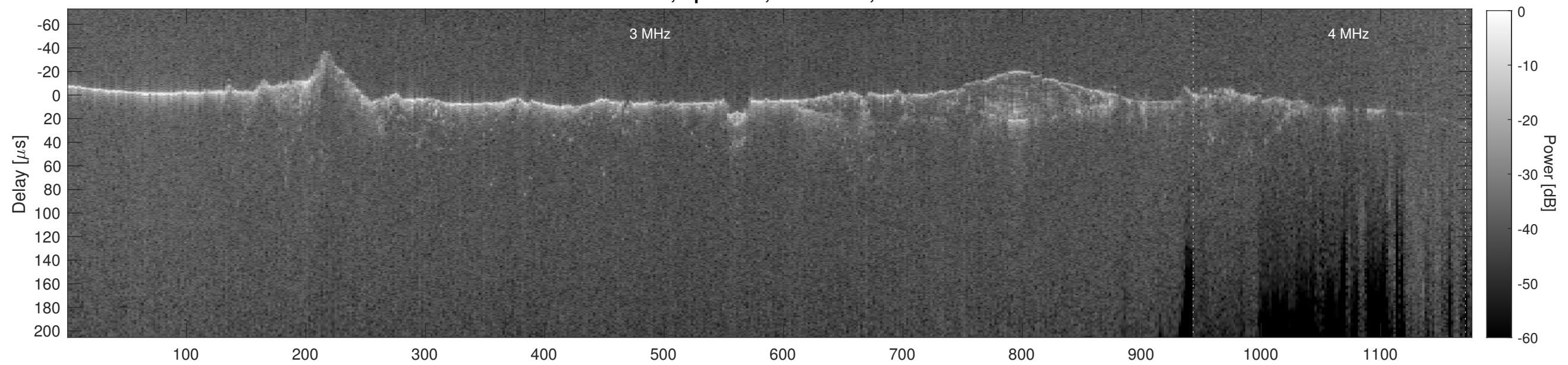
Orbit 10939, Cluttergram
