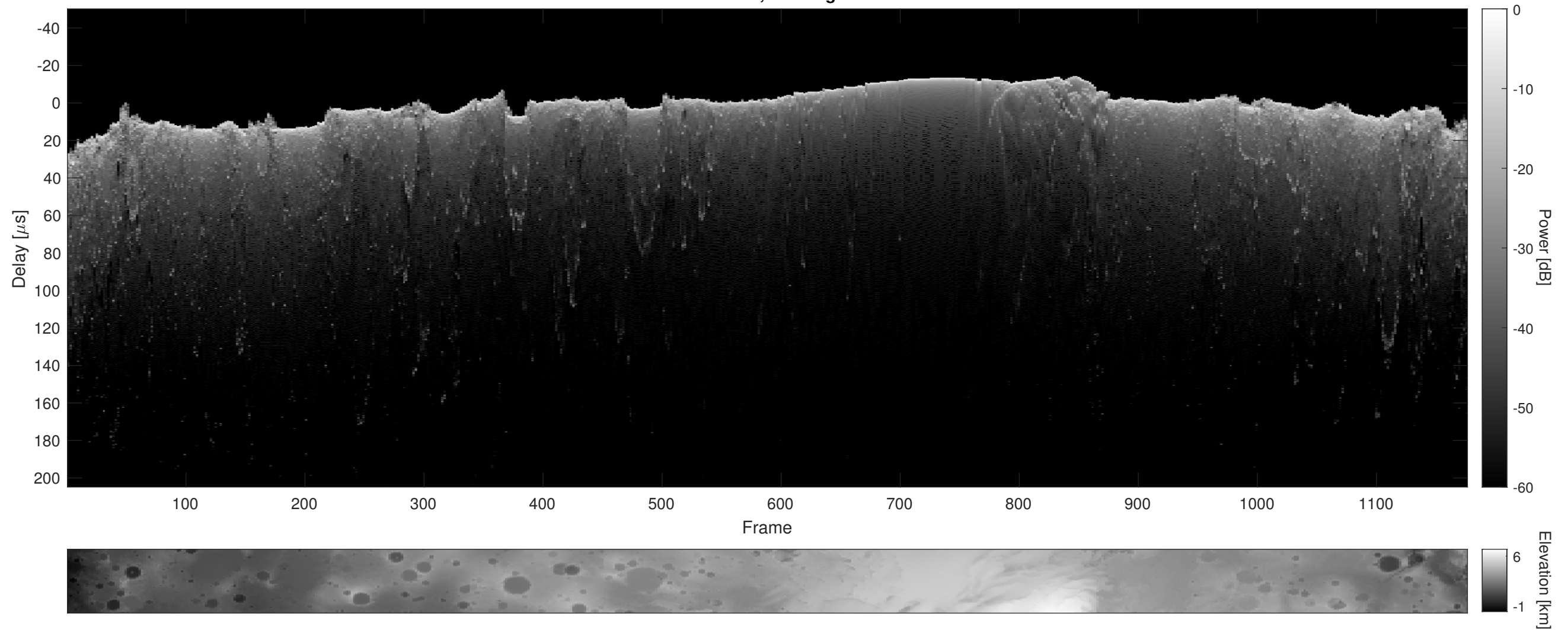
Orbit 10940, Cluttergram
