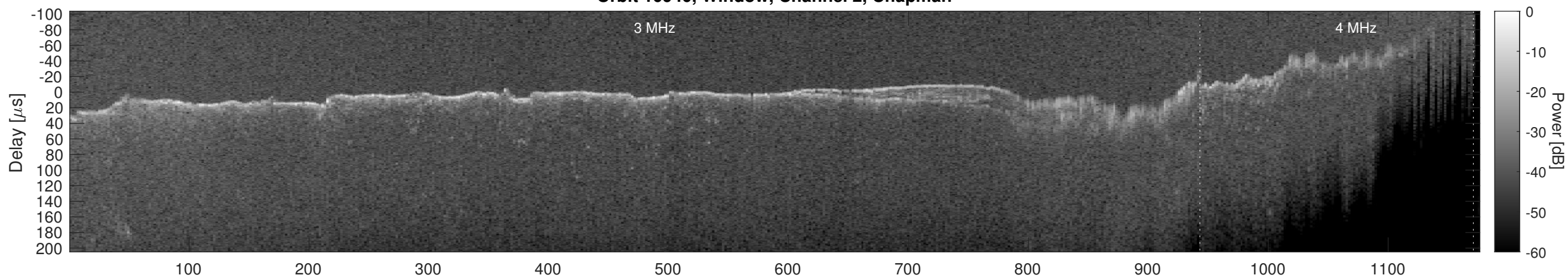
Orbit 10940, Window, Channel 2, Optimized
