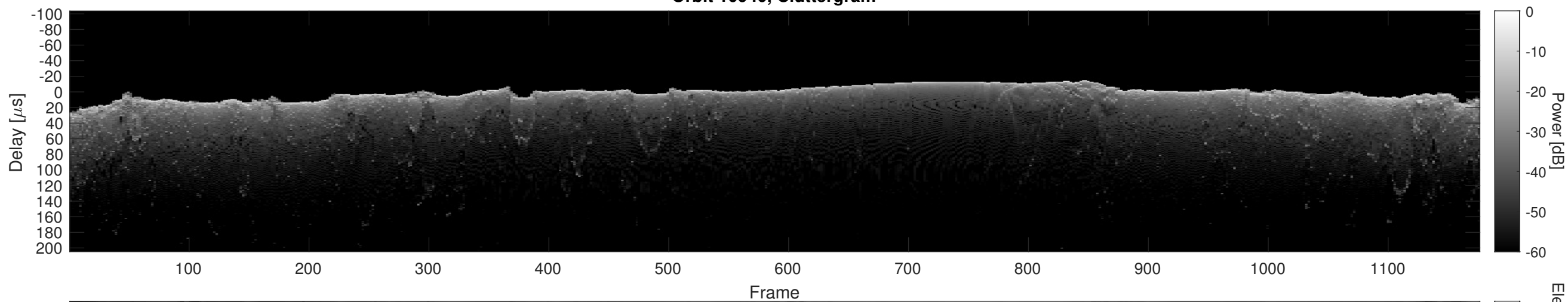
Orbit 10940, Cluttergram
