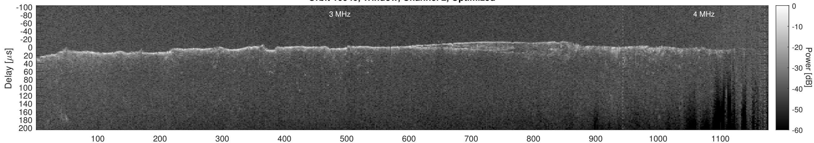
Orbit 10940, Cluttergram
