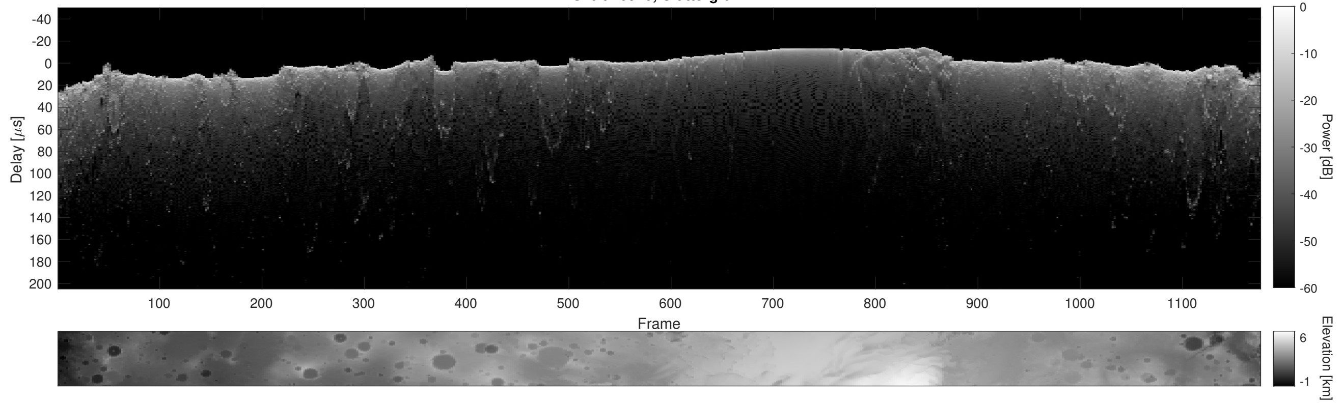
Orbit 10940, Cluttergram
