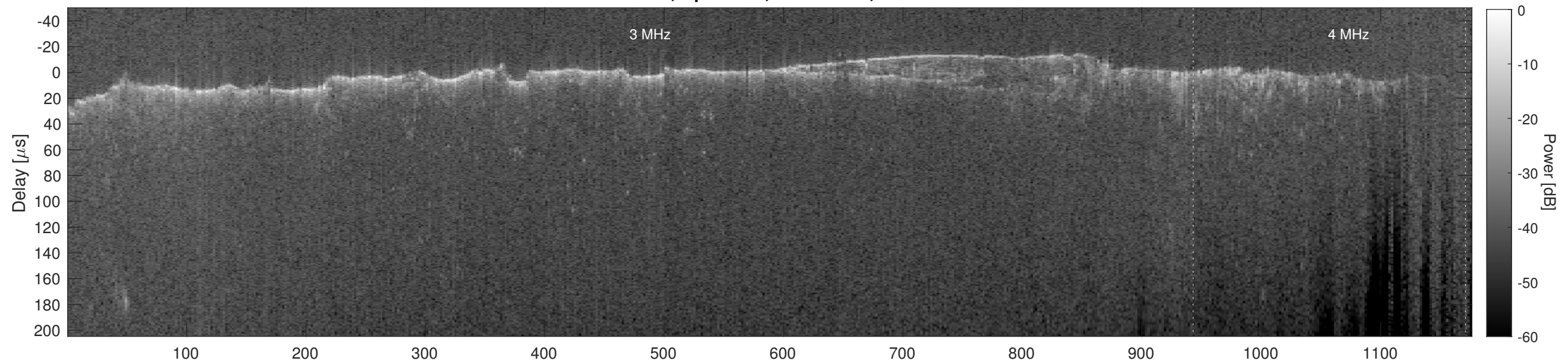
Orbit 10940, Cluttergram
