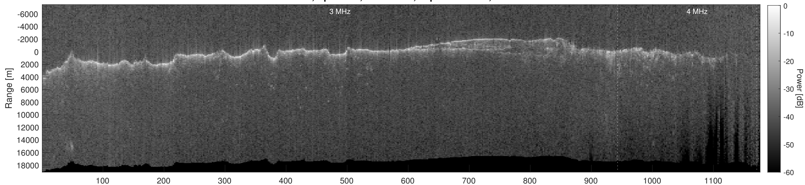
Orbit 10940, Depth-Corrected Cluttergram
