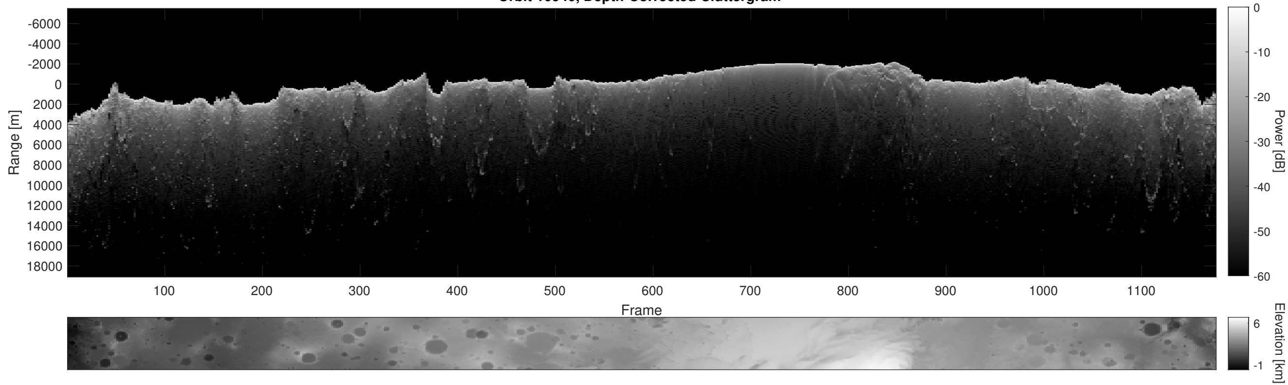
Orbit 10940, Depth-Corrected Cluttergram
