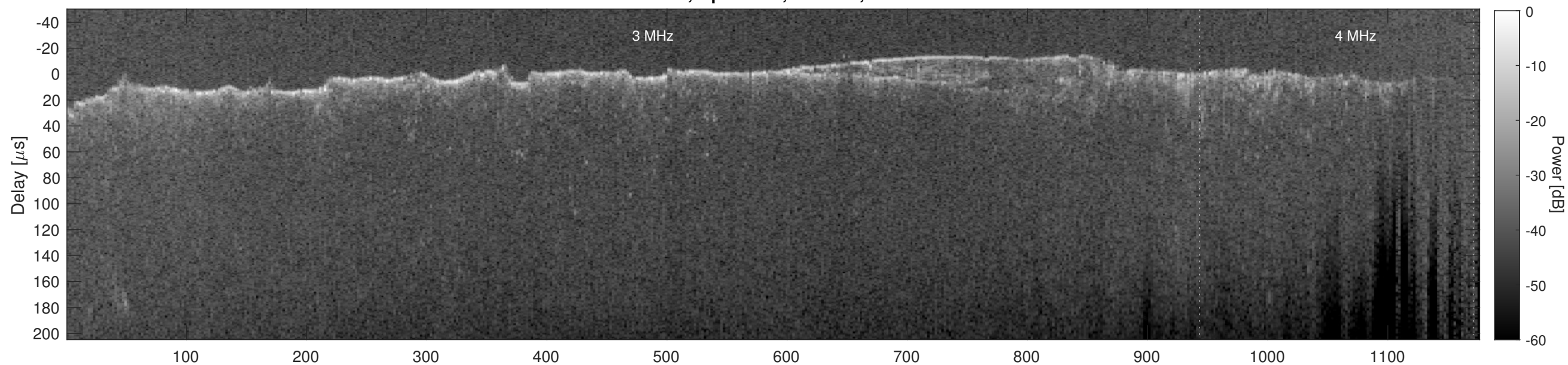
Orbit 10940, Cluttergram
