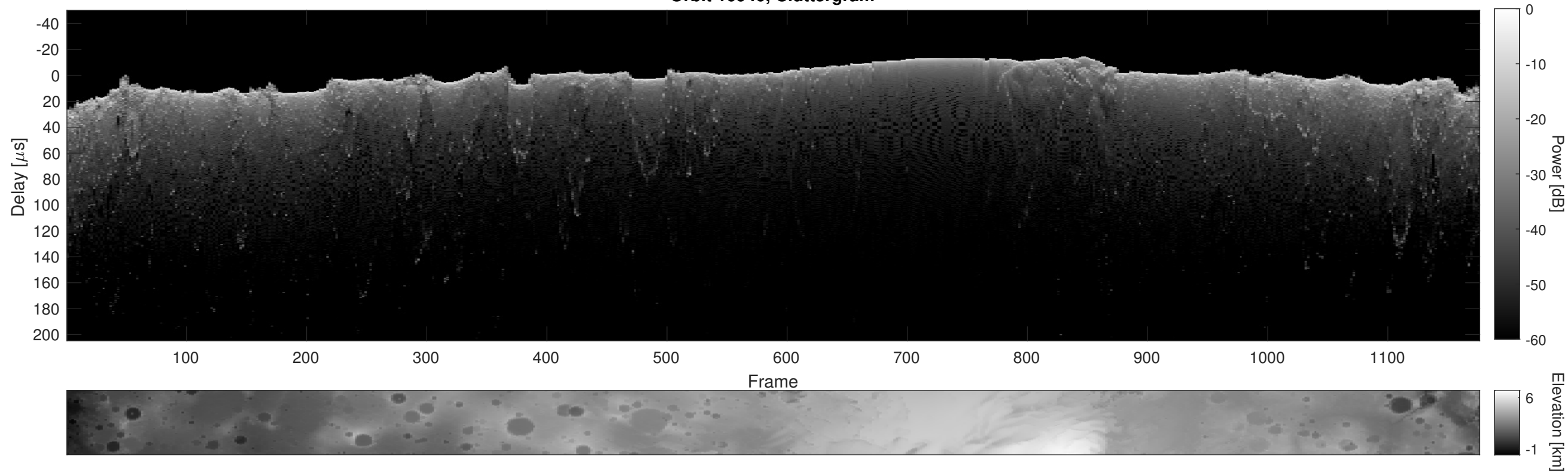
Orbit 10940, Cluttergram
